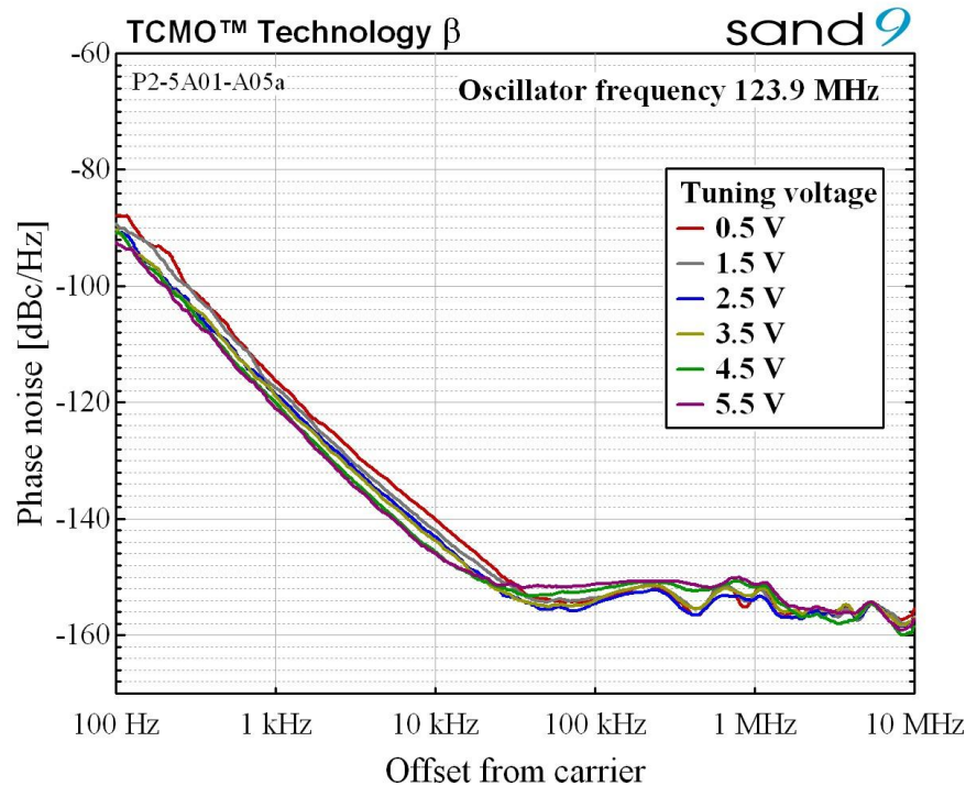
Fig. 5. Tuning voltage dependence of the single sideband phase noise of the 123.9 MHz temperature-compensated MEMS oscillator.
