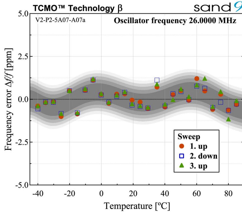
Fig. 7. Frequency error of three consecutive temperature cycles of the TCMO™ over the operating temperature range from -40^{\circ}\text{C} to +85^{\circ}\text{C} .
