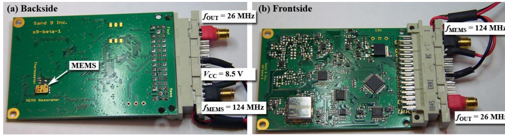
Fig. 2. Image of the beta version of the TCMO™ prototype board that is being transferred to a fully integrated solution. (a) The backside of the circuit board is comprised of the MEMS resonator in a LCC ceramic package and a temperature sensor beside it. The synthesizer and temperature control are implemented on the frontside (b).
