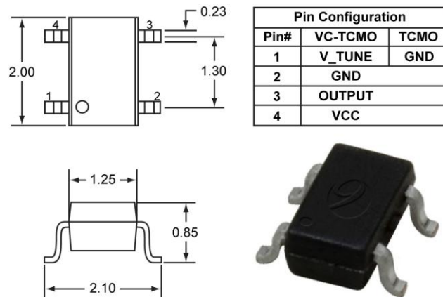
Fig. 3. Illustration of the package for the future fully integrated TCMO™. The package is similar to a 4-pin SC70 and is pin-compatible with the common universal footprints for both 2016 and 2520 TCXOs.
