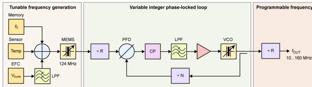
Fig. 1. Block diagram of the temperature-compensated MEMS oscillator (TCMO™) consisting of three functional blocks: tunable frequency generation, variable integer phase-locked loop, and programmable frequency output.
