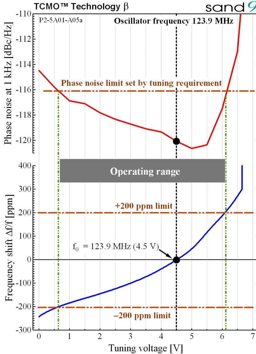
Fig. 6. Result of the frequency tuning of the MEMS oscillator and dependence of the 1 kHz phase noise versus the tuning voltage from 0 to 7 V measured with an Agilent E5052B signal source analyzer.
