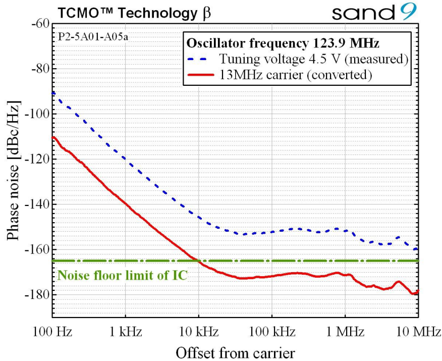
Fig. 4. Measured single sideband phase noise of the 123.9 MHz temperature-compensated MEMS oscillator (TCMO™) and phase noise converted to a 13 MHz carrier.
