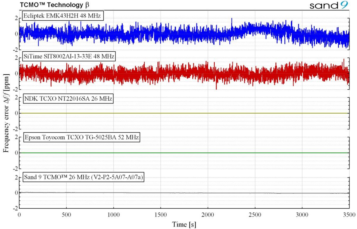
Fig. 9. Comparison of the short-term frequency stability of commercially available MEMS oscillators (Eclipsek, SiTime), quartz TCXOs (NDK, Epson Toyocom), and Sand 9's \beta -TCMO™. The large jitter observed for the MEMS oscillators originates from the fractional- N PLL, whereas the Sand 9 TCMO™ does not show this jitter, although the current beta PCB version does use a digital compensation limited by the 10-bit ADC of the temperature sensor reading. The future IC of the fully integrated TCMO™ will be entirely analog for further improvement.
