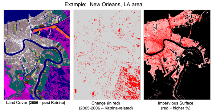
Figure 5. Land cover types, changes pre- and post- hurricane Katrina, and specific surface type products for New Orleans, Louisiana.
