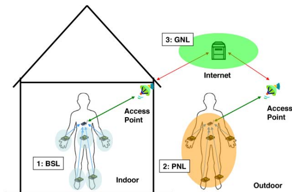
Fig. 1. The three-layer architecture of the DexterNet system: 1. Body sensor layer (BSL). 2. Personal network layer (PNL). 3. Global network layer (GNL). The pivotal component of the system is a Nokia N800 tablet at the PNL that communicates both to the BSL via IEEE 802.15.4 and the GNL via other broadband wireless channels.
