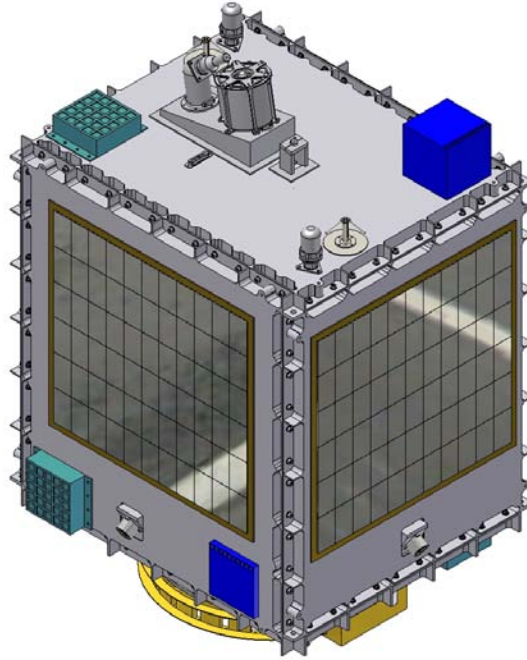
Figure 15: FalconSAT 5 showing one Solar Array for each side panel (Space Systems Research Center, 2007:4)
