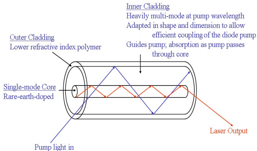
Figure 2: Fiber Laser Diagram (Perram, 2009)
