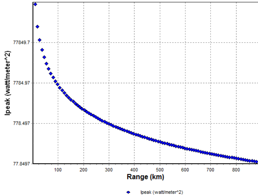
Figure 16: The Impact of Range on far field irradiance ( I_{\text{peak}} )
