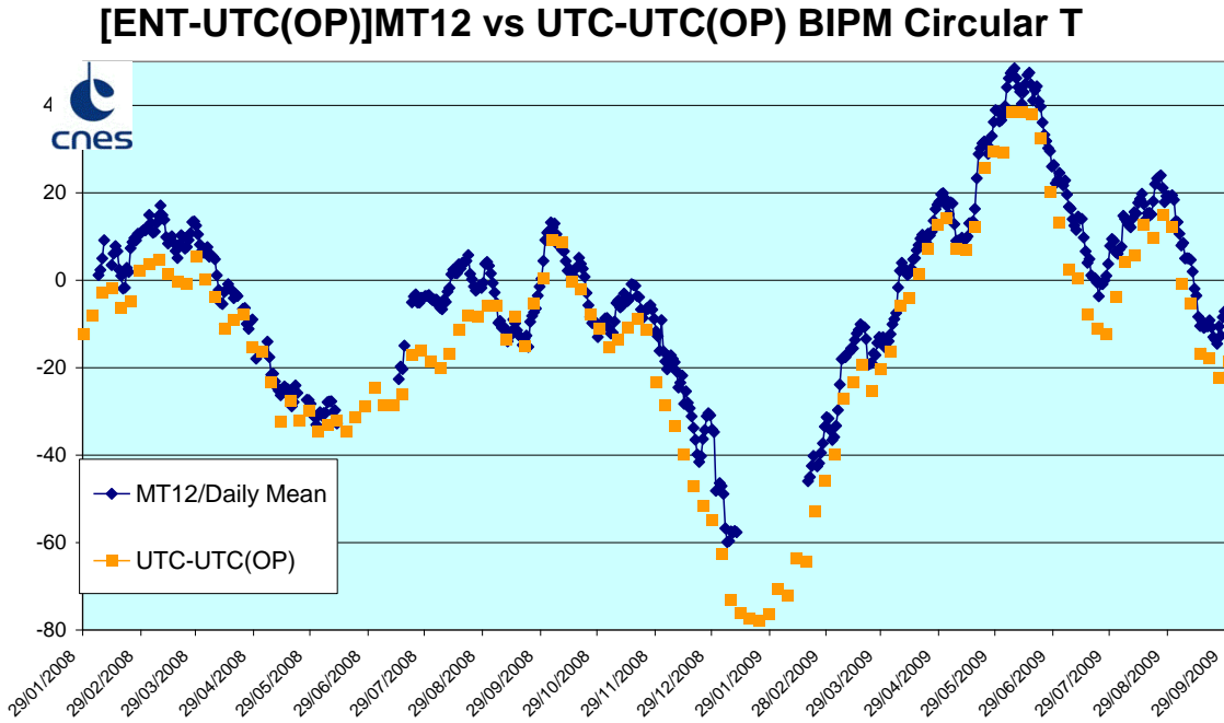
Figure 5. UTC – UTC (OP) compared to the daily mean of broadcast ENT – UTC (OP).
