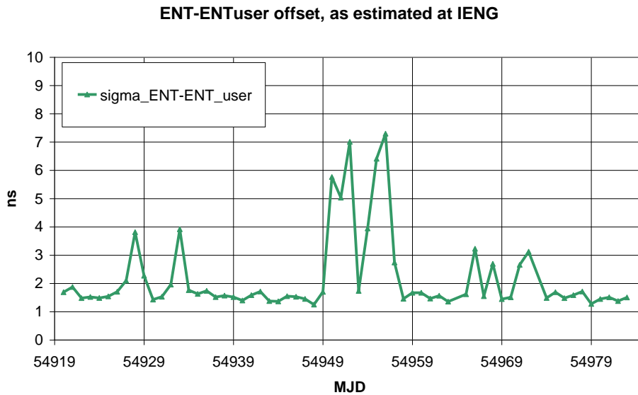
Figure 14. Standard deviation of [\text{ENT} - \text{UTC}(\text{OP})]_{\text{MT12}} - \{[\text{ENT}_{\text{user/IENG}} - \text{UTC}(\text{IT})] + [\text{UTC}(\text{IT}) - \text{UTC}(\text{OP})]\} .
