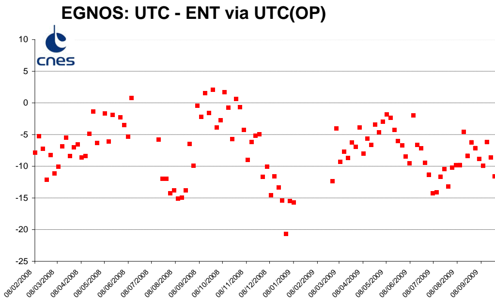
Figure 6. UTC - ENT via UTC (OP).
