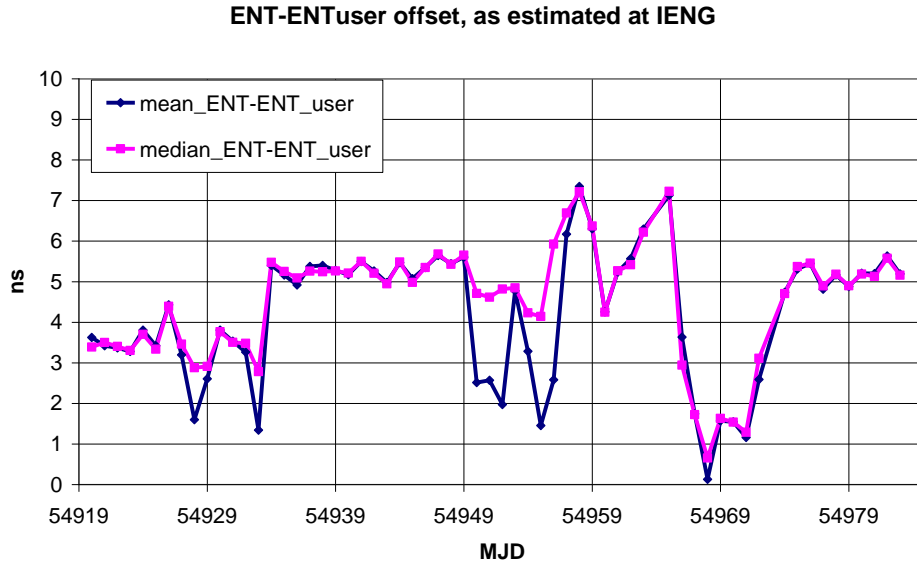
Figure 13. Daily mean and median value of [\text{ENT} - \text{UTC}(\text{OP})]_{\text{MT12}} - \{[\text{ENT}_{\text{user/IENG}} - \text{UTC}(\text{IT})] + [\text{UTC}(\text{IT}) - \text{UTC}(\text{OP})]\} .
