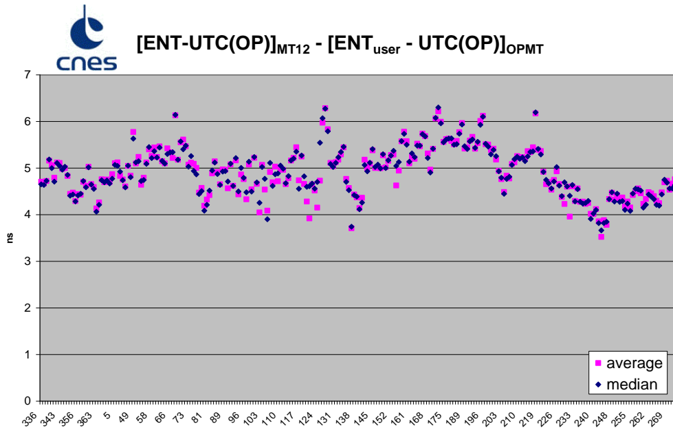
Figure 11. Daily mean and median values of [ENT - UTC (OP)]_{MT12} - [ENT_{user} - UTC (OP)]_{OPMT} .
