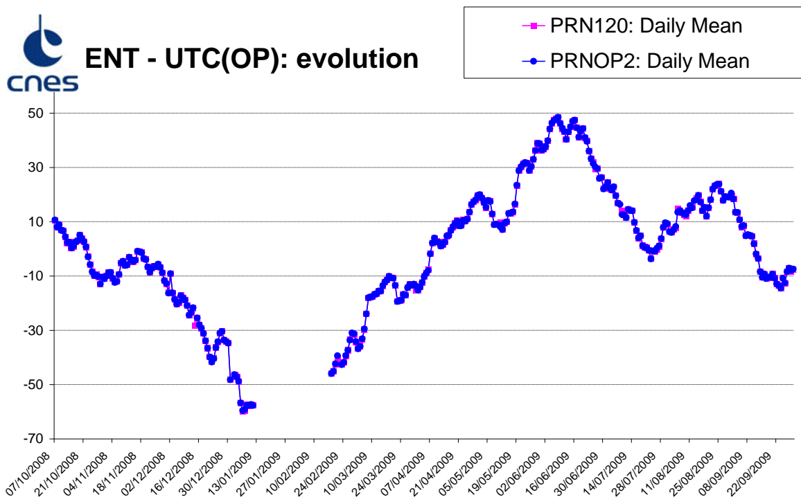
Figure 3. ENT – UTC (OP) broadcast daily means.
