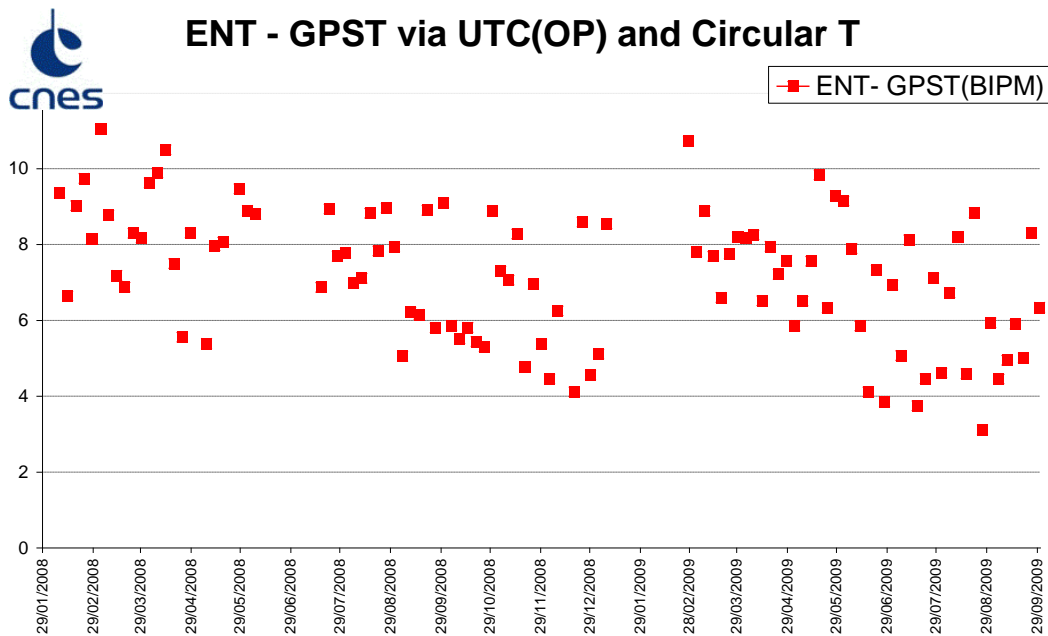
Figure 9. ENT – GPST using UTC (OP) and BIPM Circular T.
