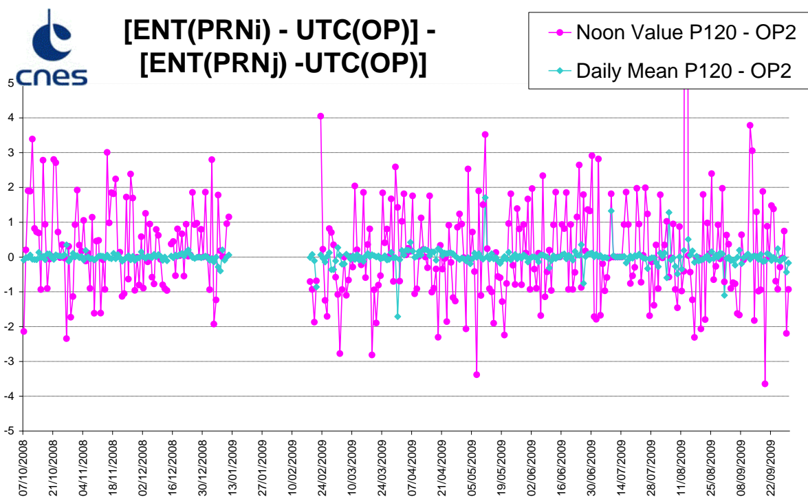
Figure 4. [\text{ENT} - \text{UTC}(\text{OP})]_{\text{PRN120}} - [\text{ENT} - \text{UTC}(\text{OP})]_{\text{PRN02}} .
