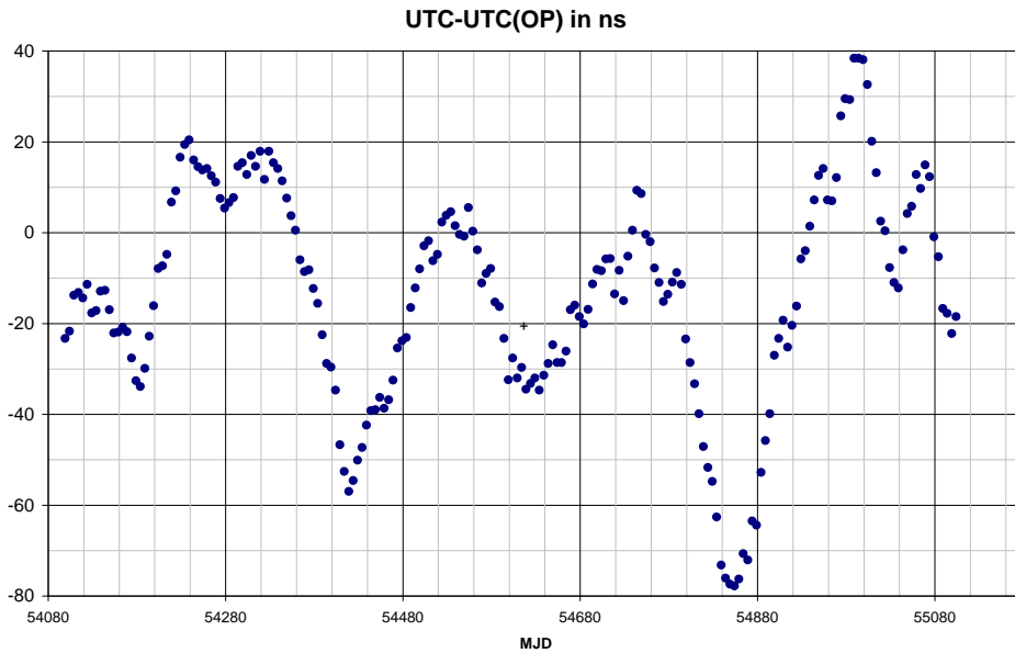
Figure 15. UTC – UTC (OP).
