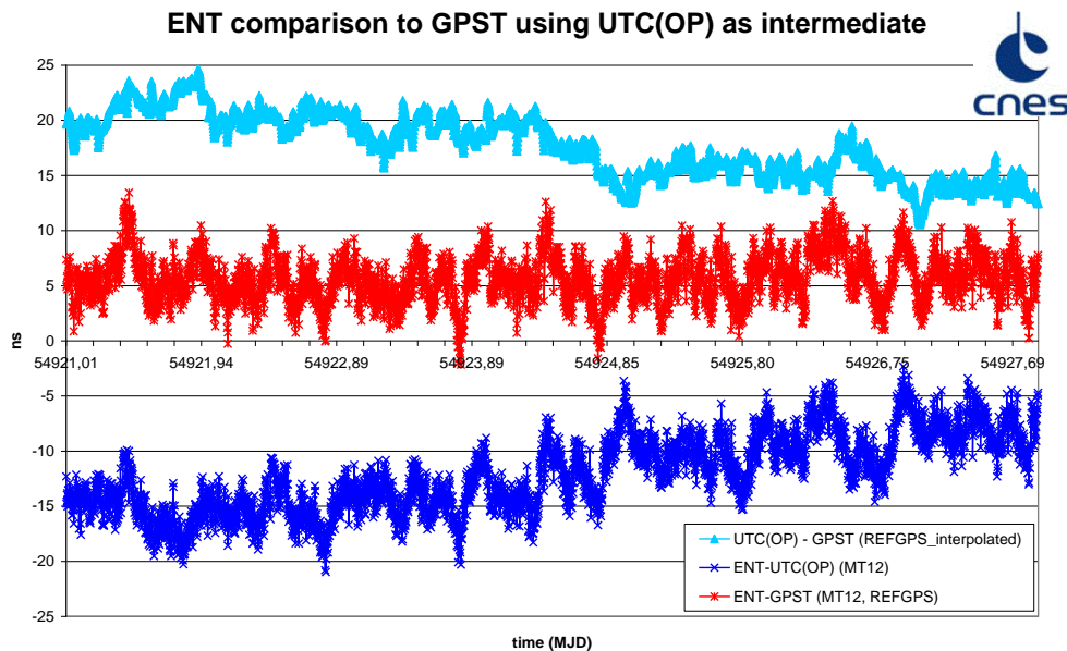
Figure 10. ENT – GPST using OP CGGTTS files.
