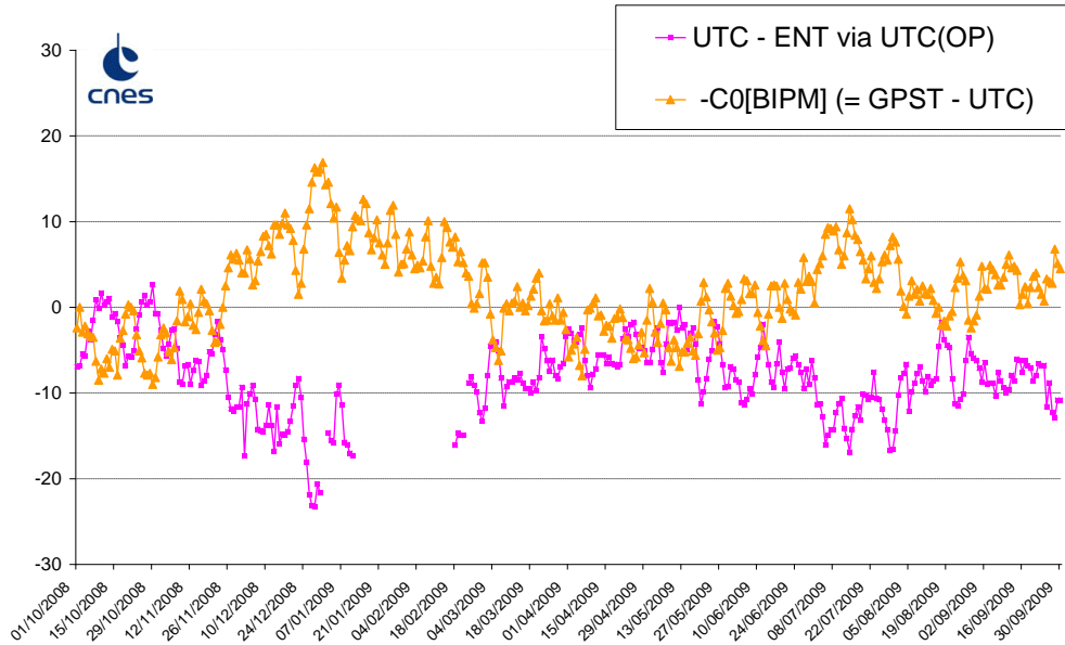
Figure 8. UTC - ENT compared to GPST – UTC.
