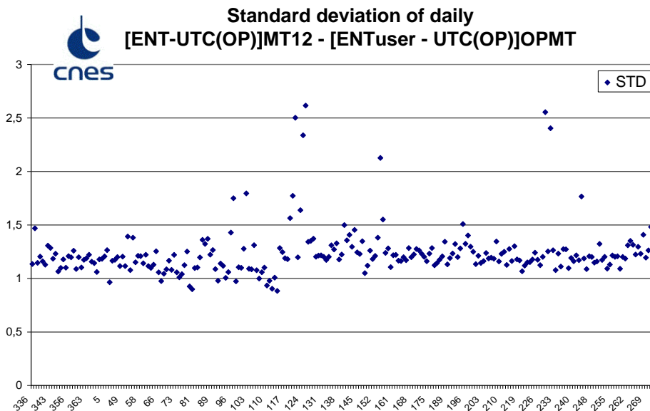
Figure 12. Daily standard deviation of [ENT - UTC (OP)]_{MT12} - [ENT_{user} - UTC (OP)]_{OPMT} .
