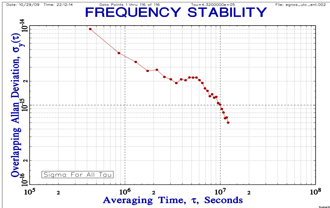
Figure 7. Allan deviation of UTC – ENT.
