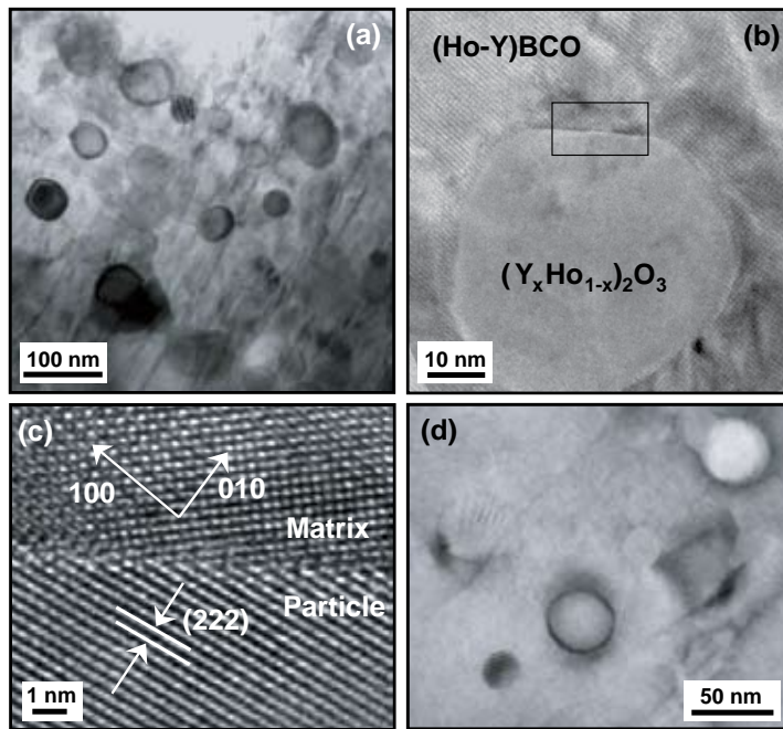
FIGURE 5 (a) A bright-field transmission electron microscopy (TEM) image showing the nanoparticles in the superconducting matrix in a Ho-doped YBCO sample. (b) A high-resolution TEM (HRTEM) image showing a coarse (Y_xHo_{1-x})_2O_3 particle. (c) A higher magnification HRTEM image showing that the particle/matrix interface of the coarse particle, obtained from the rectangular box in (b), is not fully coherent. (d) A fine particle showing the dark lobes around the particle suggesting that the particle is associated with a strain field.
