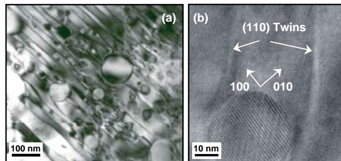
FIGURE 6 (a) A bright-field TEM image near the [001] zone of the superconducting matrix showing nanoparticles embedded in the matrix for a Ho-doped YBCO sample (lower Ho concentration than specimen of Fig. 5). Note the (110) twins. (b) HRTEM image showing the (110) twins. Note the apparent bending of twins close to the particle. Such bending could result from the interaction of strain fields present close to the particle and the twins.
