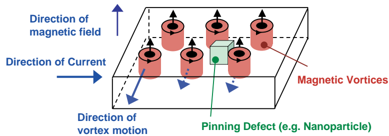
FIGURE 4 A schematic diagram illustrating the concept of pinning of the vortices by nanoparticles embedded in the superconductor.
