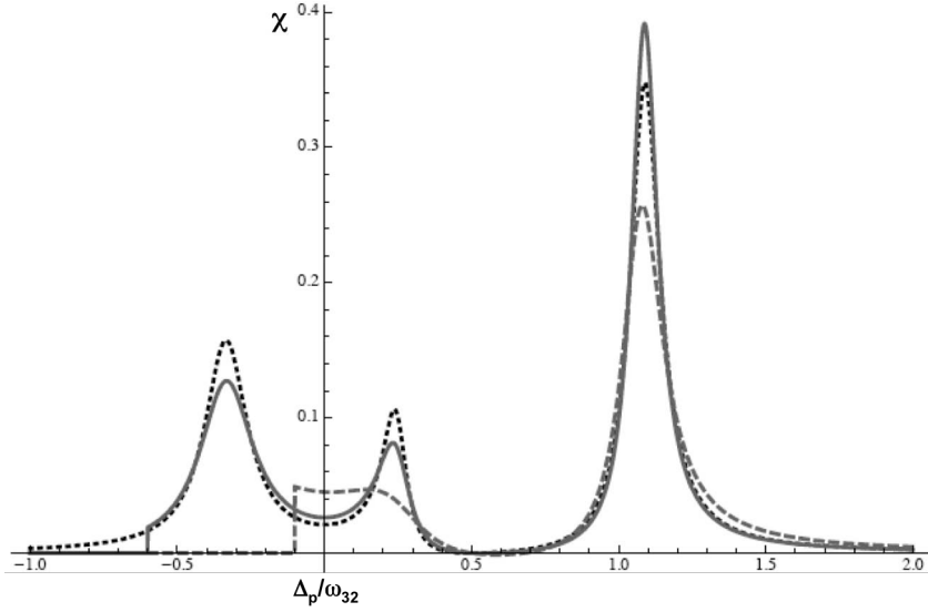
FIG. 4. Susceptibility versus pump detuning for quantized system in a cavity with g = 0.3\omega_{32} , \Delta_c = 0 , and \beta_c = 0.1\omega_{32} . The dotted curve is for a system in a cavity in free space with \bar{\gamma}_2 = \bar{\gamma}_3 = \bar{\gamma}_{23} = \bar{\gamma}_{32} = 0.05\omega_{32} . The solid and dashed curves are for a system in a PhC cavity with \beta = 0.05\omega_{32} , and \delta_g = -0.6 and \delta_g = -0.1 , respectively.
