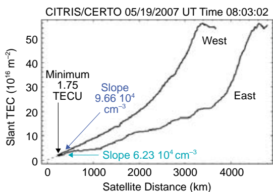
FIGURE 5 Measurements of total electron content (TEC) on the west and east side of the point of closest approach. Determination of absolute TEC uses extrapolation to zero separation between beacon and receiver satellites. The electron density is estimated from the derivative of the TEC with intra-satellite distance.
