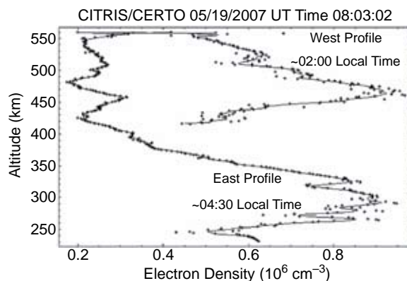
FIGURE 6 CERTO/CITRIS profiles of electron density. The dots are results of the Abel inversion with 1-km altitude separation in measured horizontal TEC. The solid line is the profile estimation using a 7-point running mean of the 1-km TEC samples.
