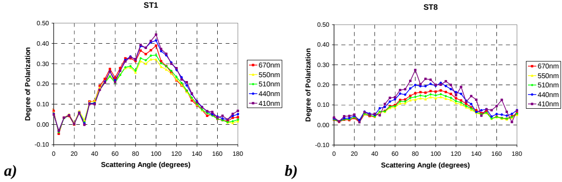
Fig. 4. Plots of the DOP vs. scattering angle. The instrument is located in the principal plane 1m below water.
