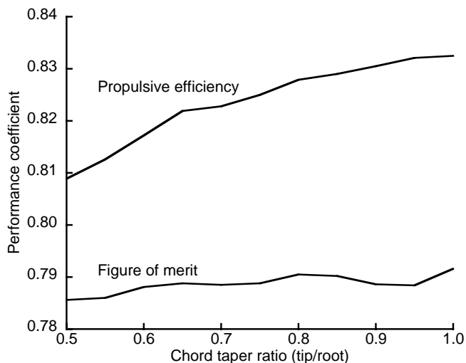
Fig. 15. Taper optimization for LCTR.
