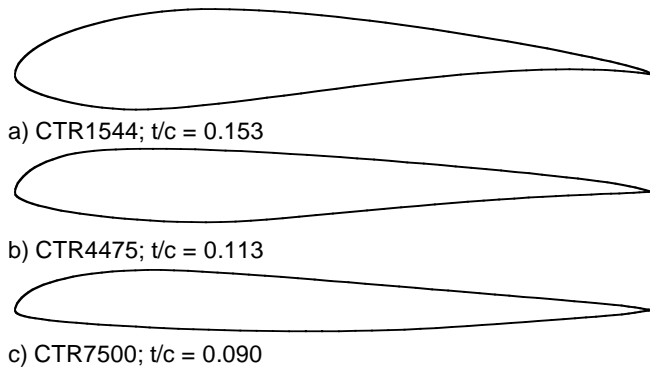
Fig. 7. LCTR airfoils.
