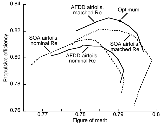
Fig. 13. LCTR twist optimization maxima for two airfoil families, for nominal and condition-matched Reynolds numbers.
