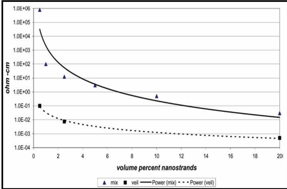
Figure 3. Solid line depicts the decrease in resistivity for a typical epoxy with the addition of nickel nanostrands TM [1].
