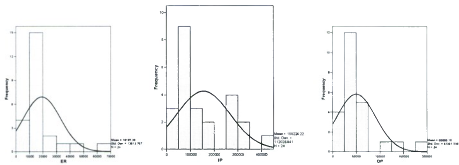
Figure C3. Histogram for patient category.
