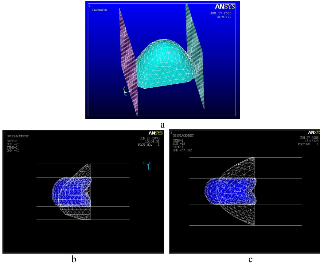
Fig. 1. Mathematical modeling and simulations of breast deformation. (a) Meshing on breast volume using FEA algorithm; (b) Simulation of CC view compression (white color: natural breast shape before compression, blue color: breast shape after compression) (c) Simulation of ML view compression (white color: natural breast shape before compression; blue color: breast shape after compression)
