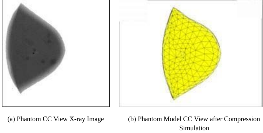
Figure 7: Comparison of Phantom X-ray Image and Simulation Result.
