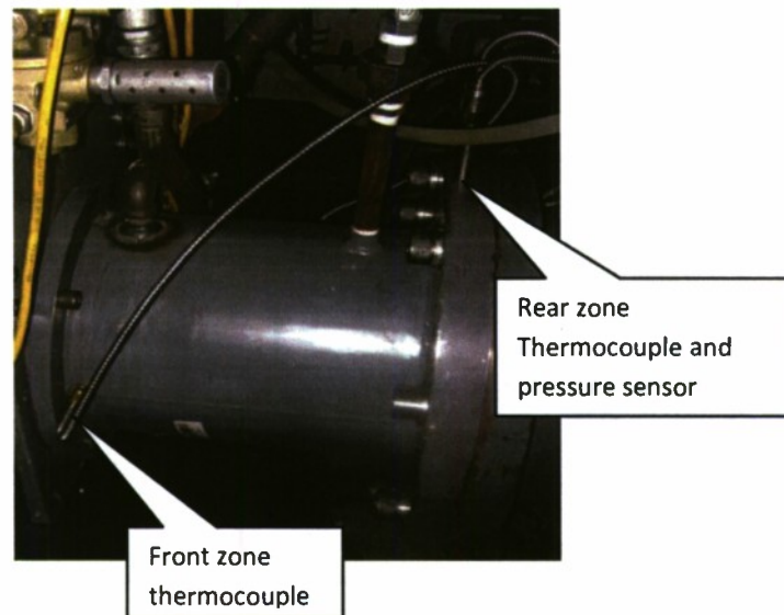
Figure 1 New extruder die installed on the existing extruder on I-Line at Milan AAP
