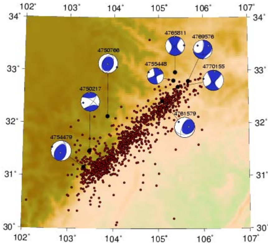
Figure 1. This figure shows the locations (small red dots) of the May 12 2008, Sichuan aftershocks from 12 May to 3 June in the Reviewed Events Bulletin from the CTBTO IDC. The total number of aftershocks shown in the figure is 1,088. Also shown are the centroid locations (larger black dots) and the MTs for eight of the aftershocks (see Table 1) for which we have a surface-wave MT inversion result. The specifications of each of the MTs shown on this figure are listed in Table 1. To link the events presented in the figure to Table 1, refer to the unique number (orid number) on top of each focal mechanism.
