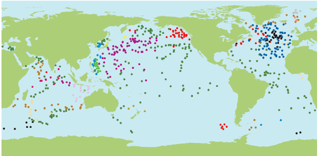
Argo Network, as of 20 January 2003 (620 Floats)
