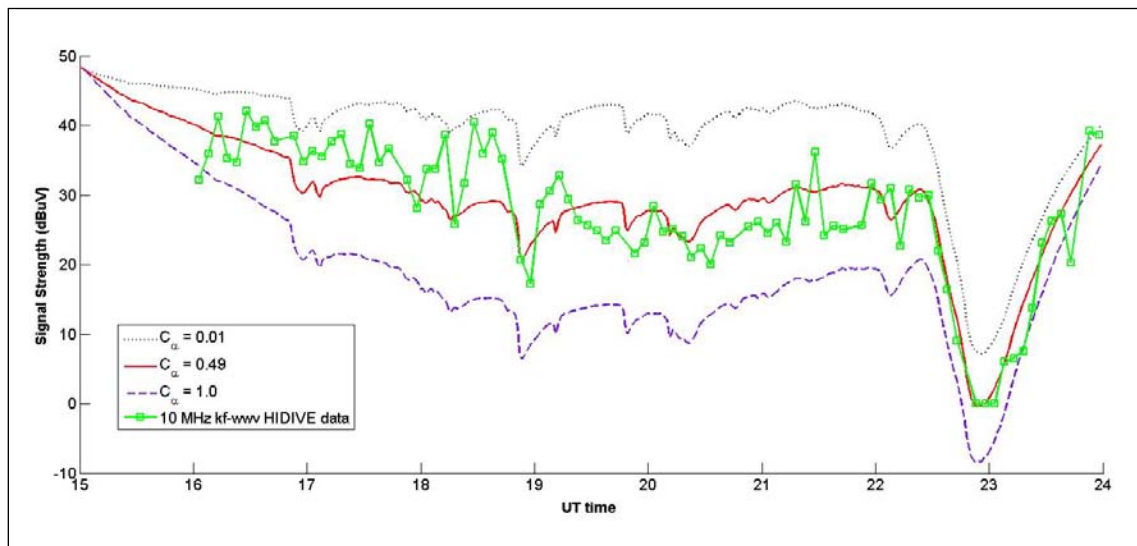
Figure 7.2.1. HIDIVE data and EHA model predictions for the 10 MHz kf-wwv signal on 15 January 2005 on which date an X2.6 flare occurred are shown. The EHA model signal strength predictions shown result from equation 7.1.6 when C_\alpha(f) equals 0.01, 0.49, and 1.0. C_\alpha(f)=0.49 results in the best fit of equation 7.1.6 to the HIDIVE data with respect to minimizing RMS error and allows for a relatively accurate prediction of flare-time signal strength.
