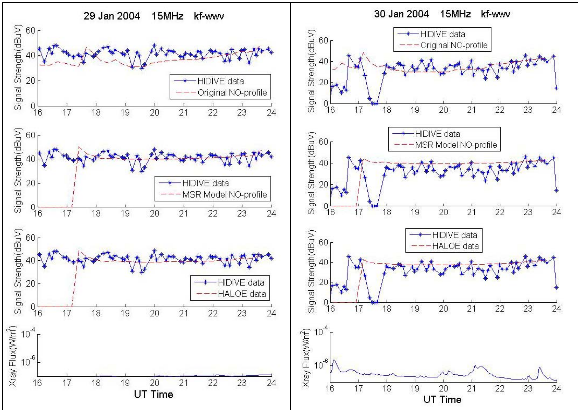
Figure F.9. HIDIVE data, GOES data, and AbbyNormal version predictions for the 15 MHz kf-www transmission on 29 January 2004.
