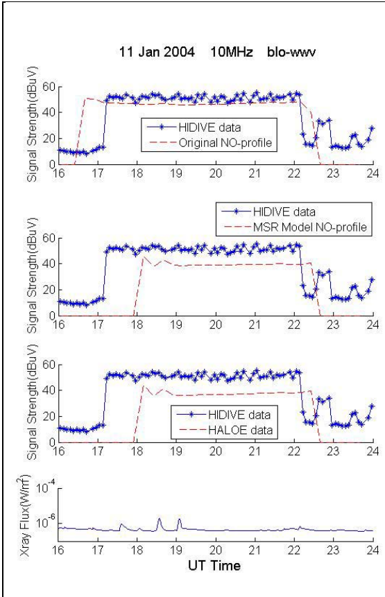
Figure C.1. HIDIVE data, GOES data, and AbbyNormal version predictions for the 10 MHz blo-wwv transmission on 11 January 2004.
