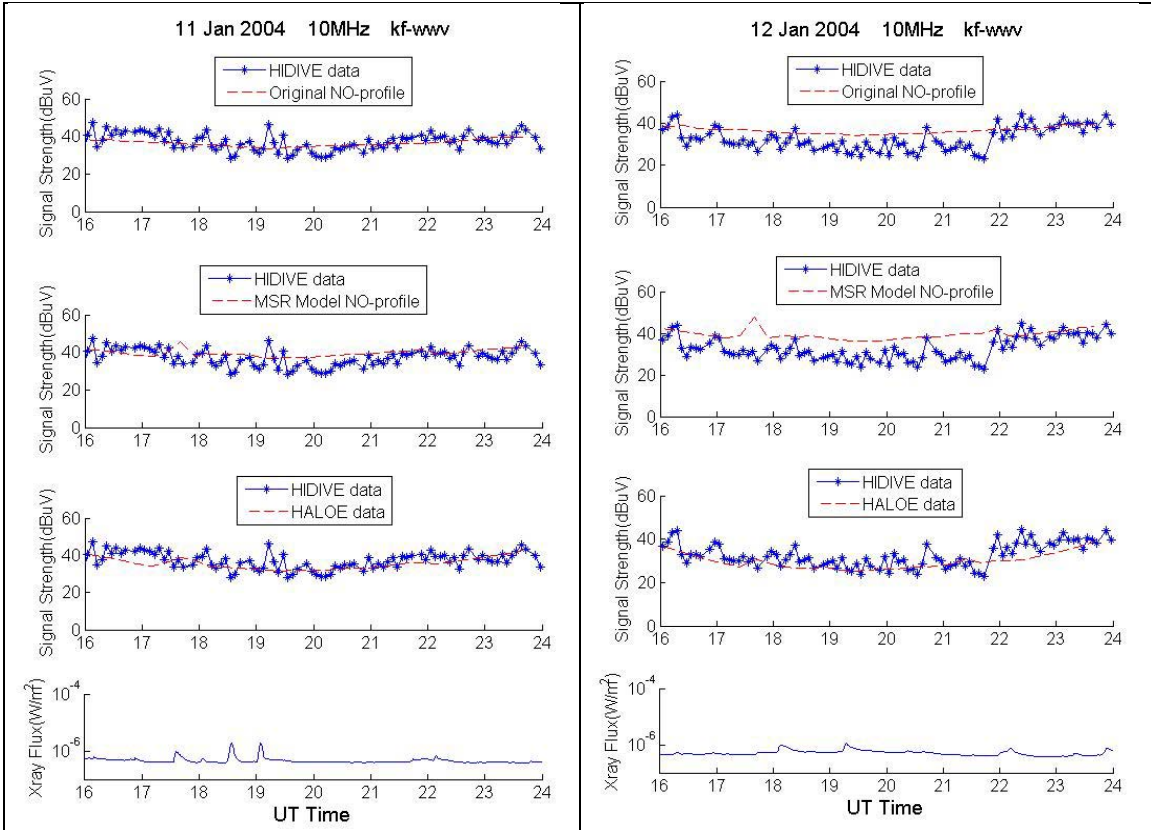
Figure E.1. HIDIVE data, GOES data, and AbbyNormal version predictions for the 10 MHz kf-wwv transmission on 11 January 2004.
