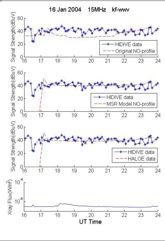
Figure F.6. HIDIVE data, GOES data, and AbbyNormal version predictions for the 15 MHz kf-wwv transmission on 16 January 2004.
