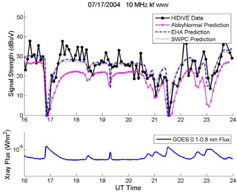
Figure A.3.2. AbbyNormal model prediction, EHA model prediction, and SWPC model prediction for the 10 MHz kf-wvv transmission on 17 July 2004 compared to HIDIVE signal strength data and GOES 0.1-0.8 nm flux data.
