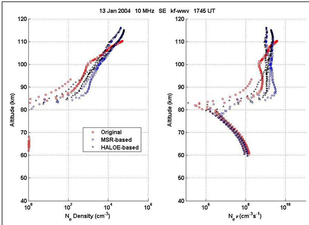
Figure 9.5.17. N_e and N_e\nu values along the raypath predicted by the AbbyNormal versions at 17:45 UT on 13 January 2004 within the D- and E-regions.
