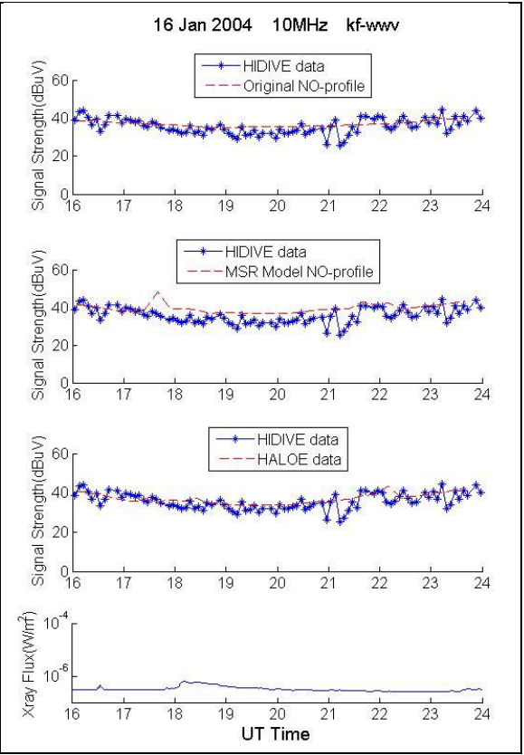
Figure E.6. HIDIVE data, GOES data, and AbbyNormal version predictions for the 10 MHz kf-wwv transmission on 16 January 2004.
