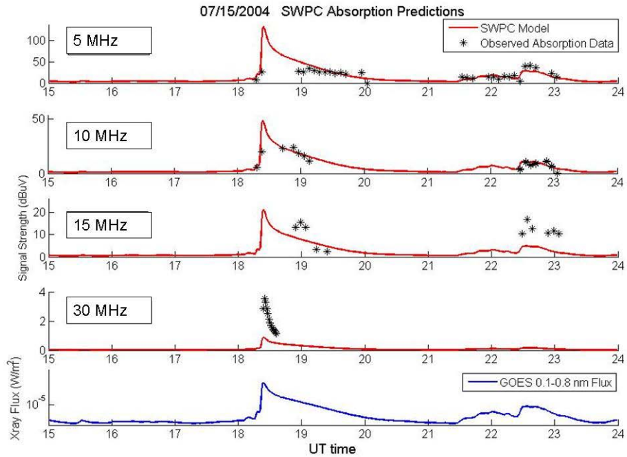
Figure 8.3.2. SWPC model predictions for X-ray induced absorption on 15 July 2004 for the 5 MHz blo-wvv signal, 10 MHz kf-wvv signal, 15 MHz kf-wvv signal, and 30 MHz riometer signal are shown along with flare-time observed absorption data.
