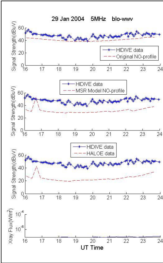
Figure B.9. HIDIVE data, GOES data, and AbbyNormal version predictions for the 5 MHz blo-wwv transmission on 29 January 2004.
