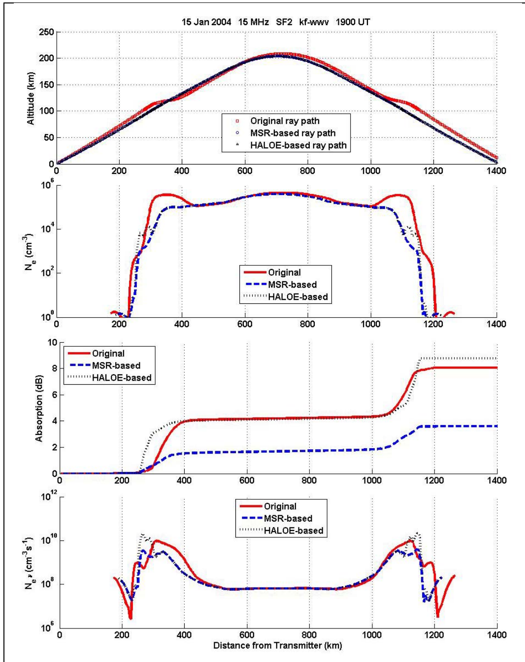
Figure 9.5.19. F-mode propagation paths predicted by HASEL for the 15 MHz kf-wwv transmission on 15 January 2004 at 19:00 UT are shown in the top panel. Also shown are the predictions of the three AbbyNormal versions of N_e along the raypath (second panel from top), total absorption suffered by the wave as it propagates (second panel from bottom), and N_e \nu along the raypath (bottom panel).
