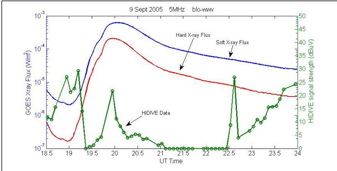
Figure 6.2.7. HIDIVE data for the 5 MHz blo-wwv transmission on 9 September 2005 are shown along with the soft and hard GOES X-ray flux. On this date, two signal strength enhancements are observed during the X6.2 flare, one at 20:00 UT and the other at 22:34 UT.
