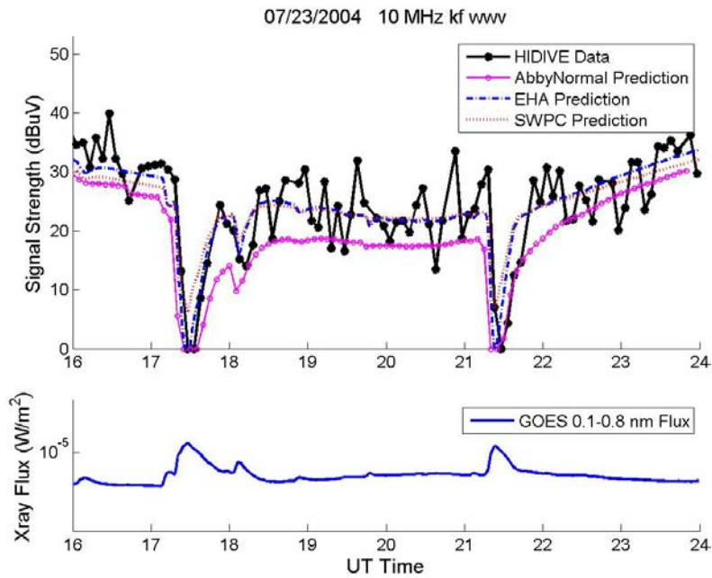
Figure A.3.3. AbbyNormal model prediction, EHA model prediction, and SWPC model prediction for the 10 MHz kf-wvv transmission on 23 July 2004 compared to HIDIVE signal strength data and GOES 0.1-0.8 nm flux data.
