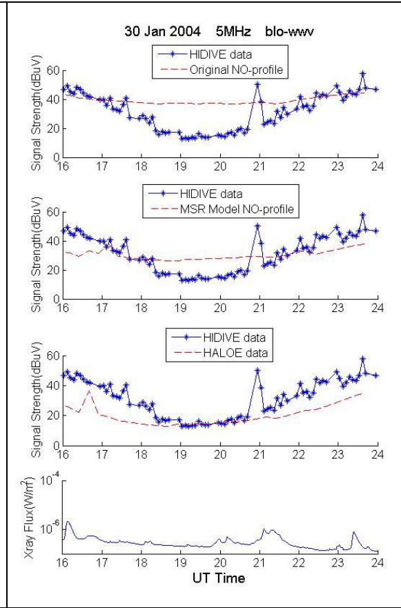
Figure B.10. HIDIVE data, GOES data, and AbbyNormal version predictions for the 5 MHz blo-wwv transmission on 30 January 2004.
