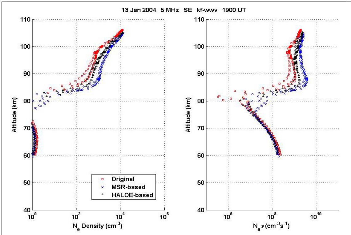
Figure 9.5.10. N_e and N_e v values along the raypath predicted by the three AbbyNormal versions for 13 January 2004.
