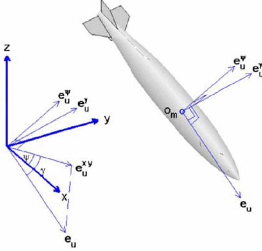
Figure 9. Unit vectors ( \mathbf{e}_u , \mathbf{e}_u'' , \mathbf{e}_u' , \mathbf{e}_u^{xy} ) [From Chu et al. 2010]
