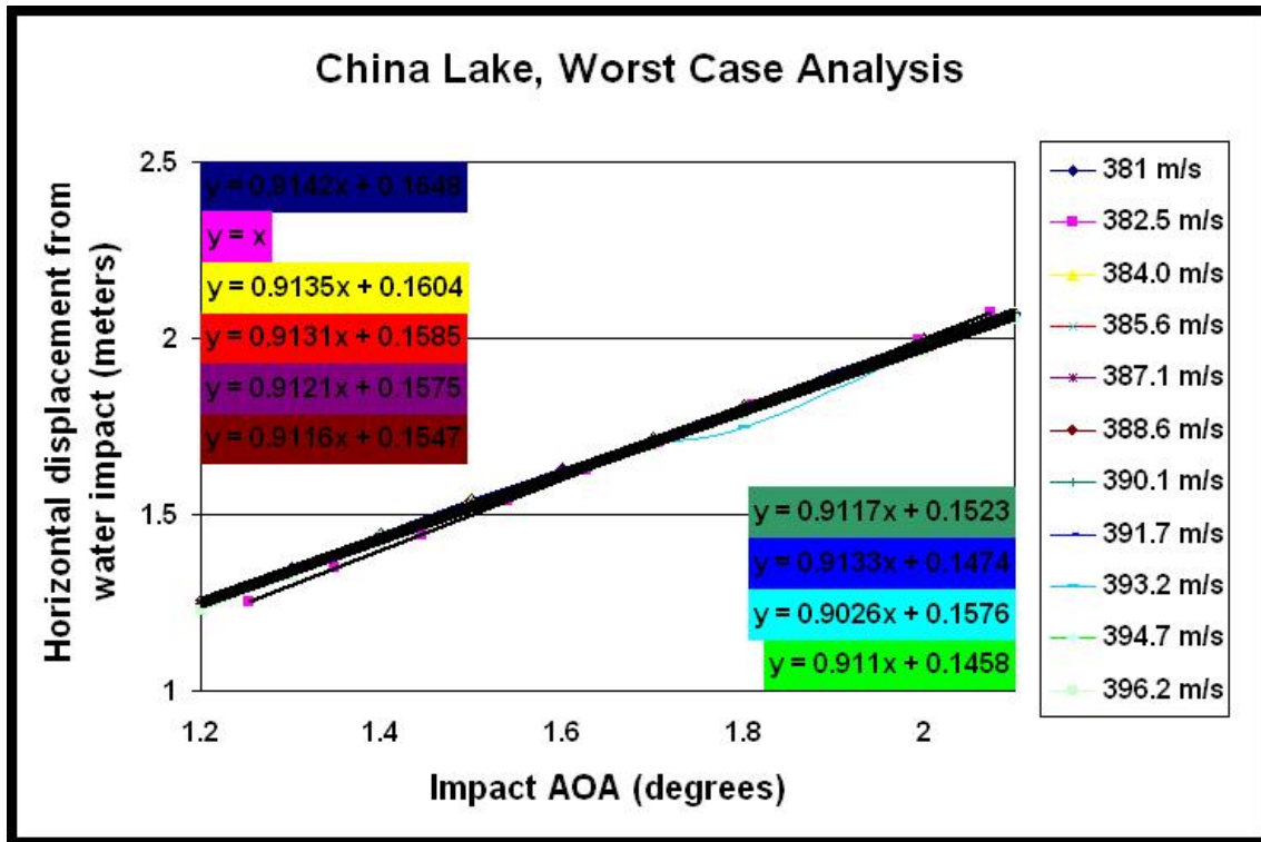
Figure 46. Most impact speeds have almost linear horizontal displacement between about 1.2^\circ and 2.1^\circ
