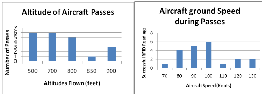
Figure 12. Altitude and Ground Speed of the Aircraft During Passes
