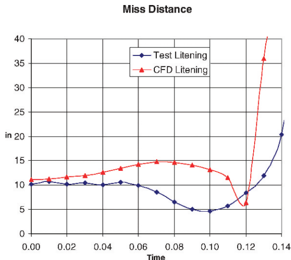
Figure 4. Fuel tank miss distance at M = 0.95 .
