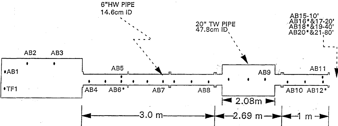
Figure 5. Small-scale magazine model with in-line expansion chamber; Series 2, layout for Tests 73, 74, and 75, chamber loading densities are 1.67, 3.33, and 5.00 kg/m 3 , respectively.
