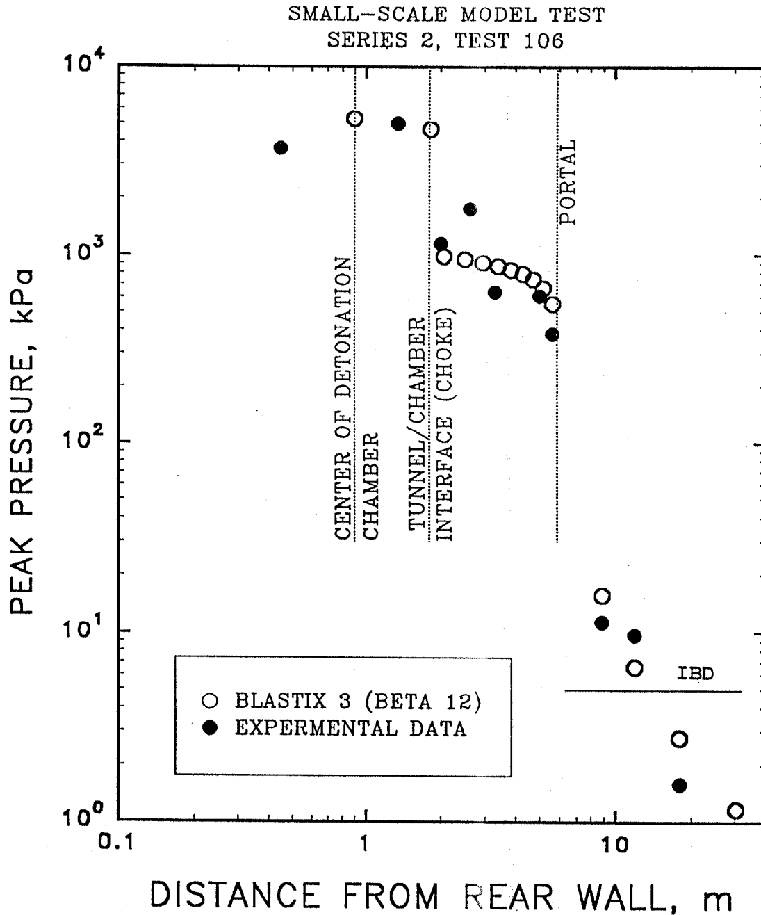
Figure 12. Comparison of measured peak overpressure from small-scale shot-gun magazine model with constriction (Series 2, Test 106) and BLASTX3 computed data, chamber loading density of 5.0 kg/m 3 .
