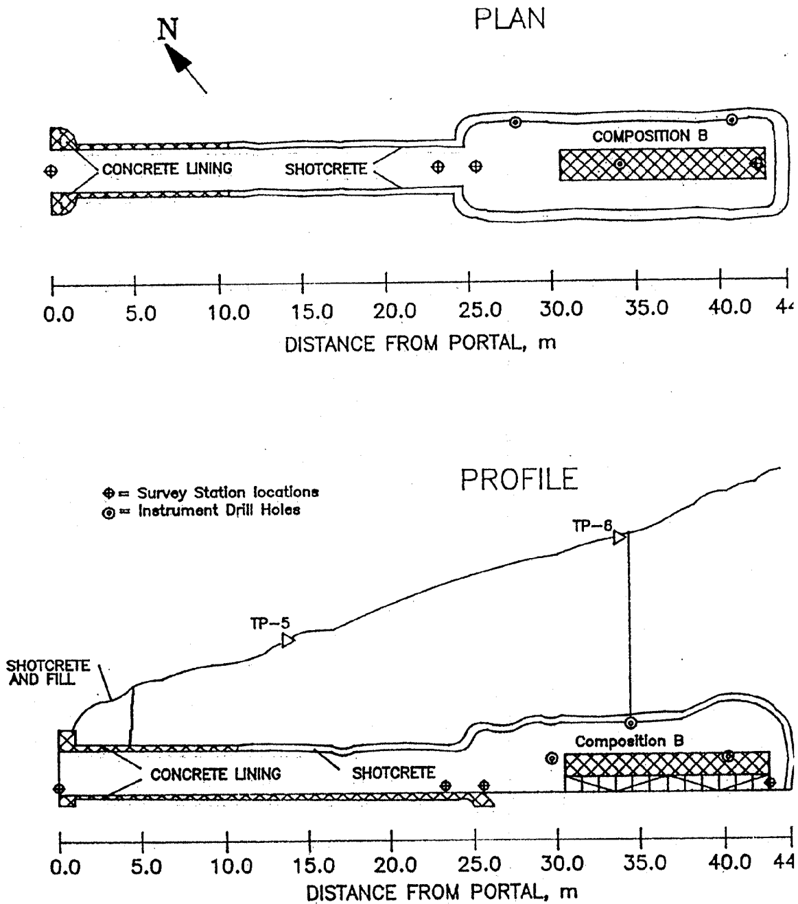
Figure 17. Large-scale shallow underground magazine test; KLOTZ 1988 test layout at China Lake, chamber loading density of 66.4 \text{ kg/m}^3 .
