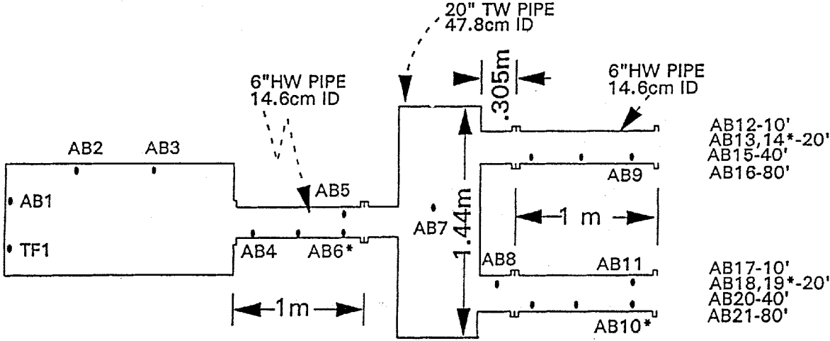
Figure 9. Small-scale magazine model with a transverse dual exit expansion chamber; Series 2, Test 82 layout, chamber loading density of 5.00 kg/m 3 .
