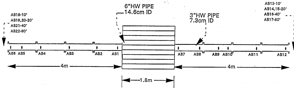
Figure 13. Small-scale magazine model with dual exits (opposing) ; Series 2, Test 113 layout, chamber loading density of 15.0 kg/m 3 .
