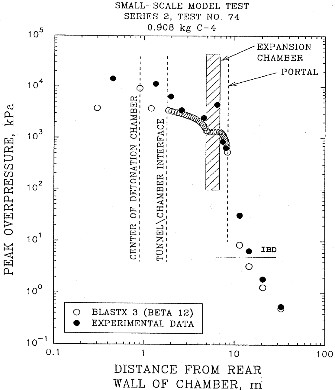
Figure 7. Comparison of measured peak overpressure from small-scale magazine model with in-line expansion chamber (Series 2, Test 74) and BLASTX3 computed data, chamber loading density of 3.33 \text{ kg/m}^3 .
