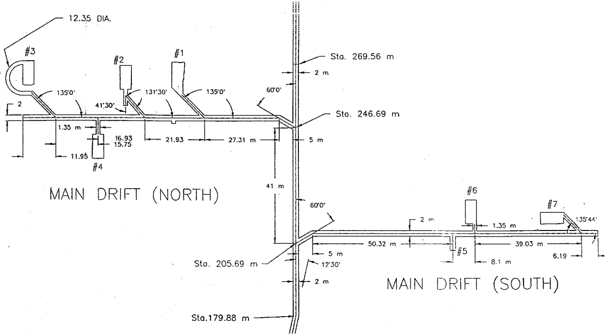
Figure 23. Joint US/ROK R&D Program, Intermediate-Scale Underground Magazine Tests in the Linchburg Mine, test layout, Chamber No. 4 loading densities of 1.1, 5.5, 14.6, and 37.3 kg/m 3 .
