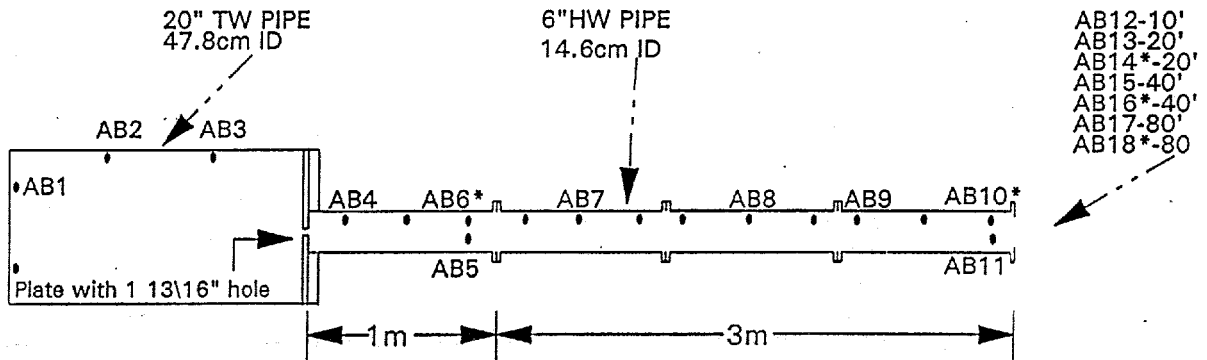
Figure 11. Small-scale shot-gun magazine model with constriction; Series 2, Test 106 layout, chamber loading density of 5.0 kg/m 3 .
