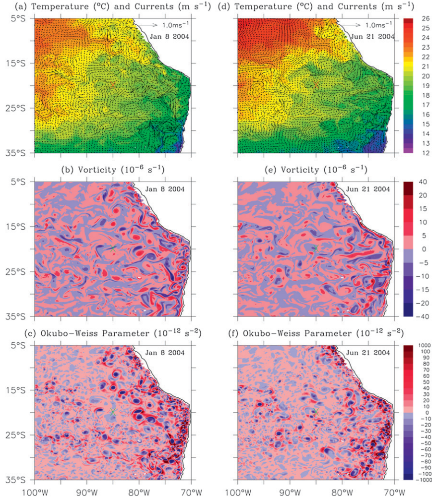
FIG. 10. Ocean states at 30 m in HYCOM on two dates. (a) Temperature (shading contours in ^{\circ}\text{C} ) and currents (vectors in \text{m s}^{-1} ), (b) relative vorticity (in 10^{-6} \text{ s}^{-1} ), and (c) OWP ( 10^{-12} \text{ s}^{-2} ) on 8 Jan 2004. (d),(e),(f) As in (a),(b),(c), but on 21 Jun 2004. The color bars on right are for (top) temperature, (middle) vorticity, and (bottom) OWP.
