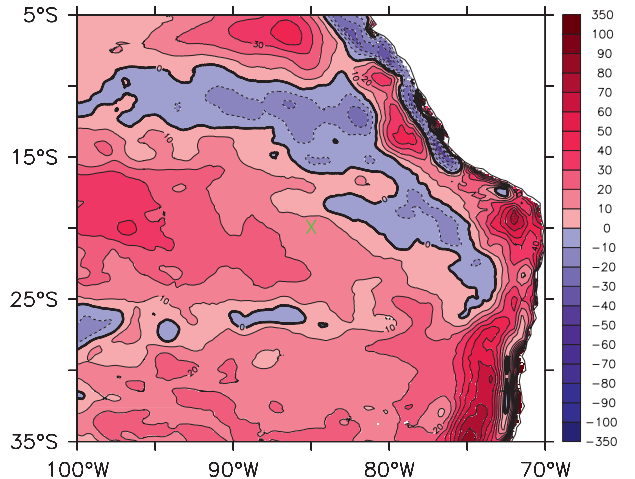
FIG. 3. Mean net surface heat flux ( \text{W m}^{-2} ; downward positive) based on NOGAPS and HYCOM SST averaged over 2003–07. The IMET site is marked by a green X on the map.
