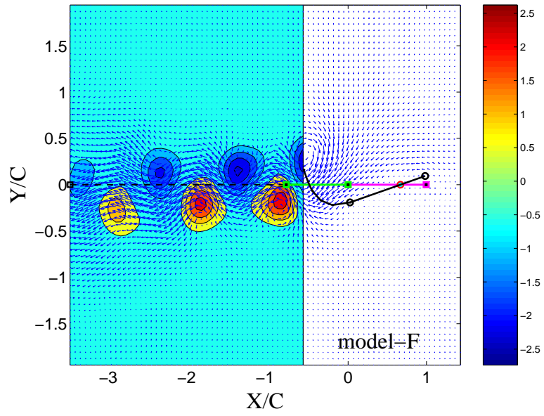
Figure 4: Ensemble average velocity and vorticity field when the rigid trailing edge is at bottom-extreme location: model-F.
