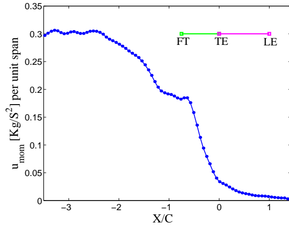
Figure 10: Variation of mom_X in downstream direction for model-F.
