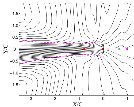
Figure 12: Streamlines around model-F, from the mean flow field. The dotted lines above and below the mean-position line indicate the jet-envelopes.
