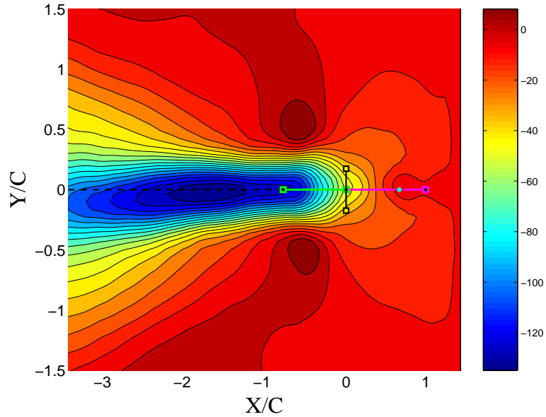
Figure 7: Iso-contours of velocity in X-direction ( u ) : model-F.
