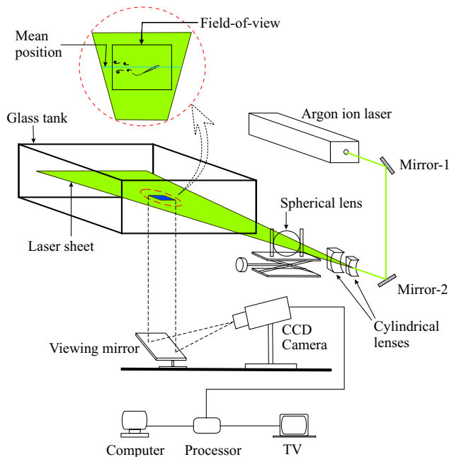
Figure 3: Schematic illustrating optics arrangement.
