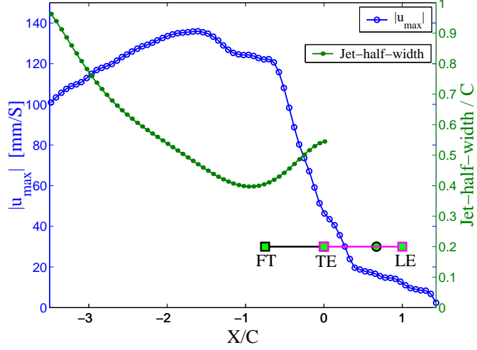
Figure 8: Variation of the maximum u -velocity and jet half-width in the downstream direction.
