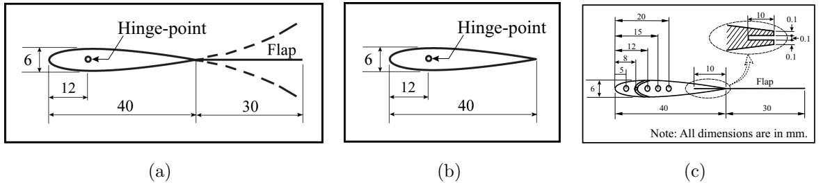
Figure 2: Schematic sectional views of the airfoil models: (a) model-F, (b) model-R, (c) details of model-F. All dimensions are in mm.
