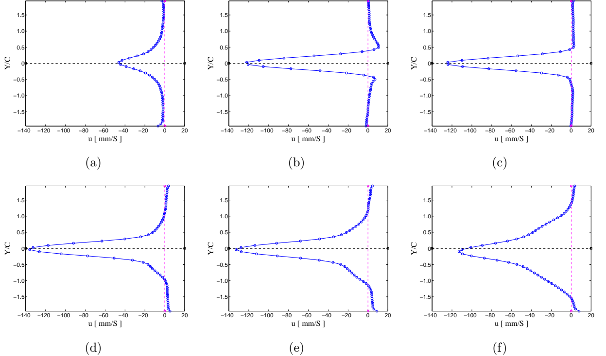
Figure 9: u -velocity profiles at some specific downstream locations; model-F: (a) \frac{X}{C} \approx 0 , at trailing edge (b) \frac{X}{C} \approx -0.76 , close to flap tip location in mean-position, (c) \frac{X}{C} \approx -1 , (d) \frac{X}{C} \approx -1.61 , highest u_{max} location, (e) \frac{X}{C} \approx -2 , (f) \frac{X}{C} \approx -3 .
