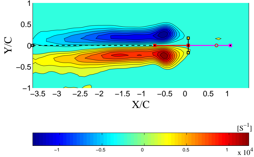
Figure 6: Average vorticity from mean flow field: model-F.
