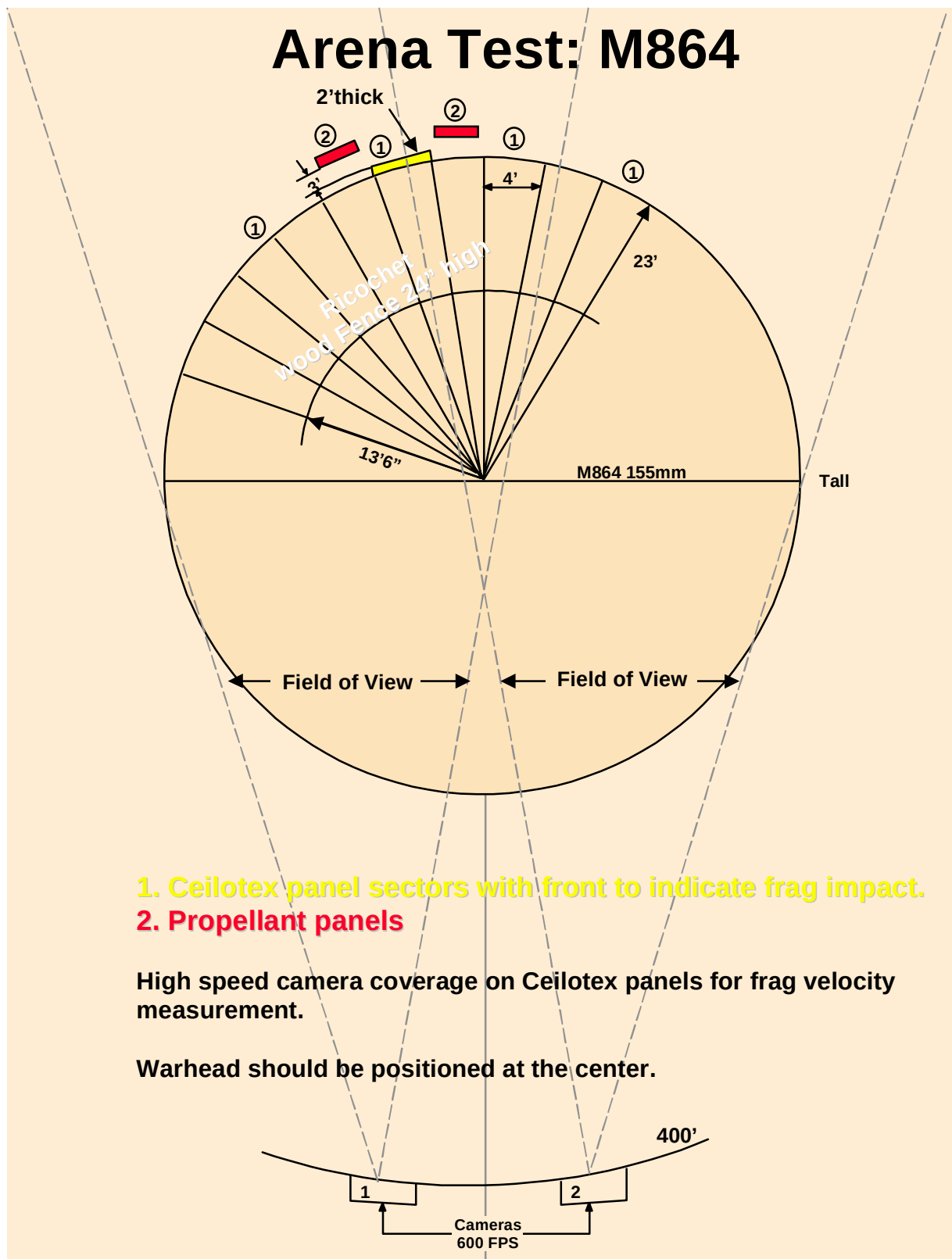
Figure 7. Schematic of M864 Arena Test.
