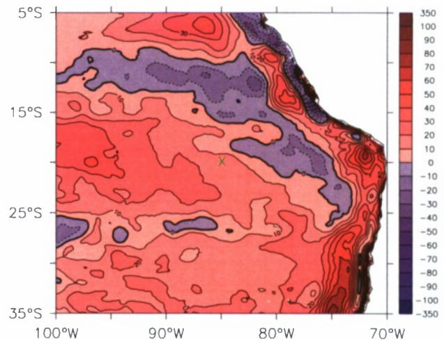
FIG. 3. Mean net surface heat flux ( \text{W m}^{-2} ; downward positive) based on NOGAPS and HYCOM SST averaged over 2003–07. The IMET site is marked by a green X on the map.
