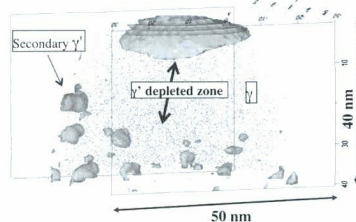
Fig. 3—(Color online) A 50 \times 50 \times 40 -nm 3DAP reconstruction from the same SC0 sample as in Fig. 2, showing Al ions (in red) and a Cr isococoncentration surface (also referred to in short as isosurface) for Cr = 14 at. pct (in blue). This reconstruction contains a portion of primary \gamma' precipitate and a number of secondary \gamma' precipitates.
