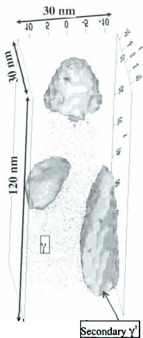
Fig. 6—(Color online) A 30 \times 30 \times 120 -nm 3DAP reconstruction from SC50 sample, showing Al ions (in red) and a Cr isocentration surface (also referred to in short as isosurface) for Cr = 14 at. pct (in blue). This reconstruction contains substantial portions of secondary \gamma' precipitates.
