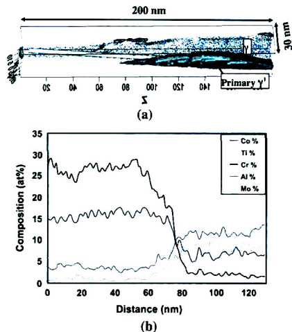
Fig. 5—(Color online) (a) A 30 \times 30 \times 200 -nm 3DAP reconstruction from SC50 sample, showing Al ions (in red) and a Cr isosurface (also referred to in short as isosurface) for Cr = 14 at. pct (in blue). Reconstruction contains a section of a large primary \gamma' precipitate as well as some sections of smaller secondary \gamma' precipitates. On it is superimposed a cylinder 5 nm in diameter along which a composition profile has been obtained. (b) Corresponding composition profile for Cr, Co, Al, Ti, and Mo ions.
