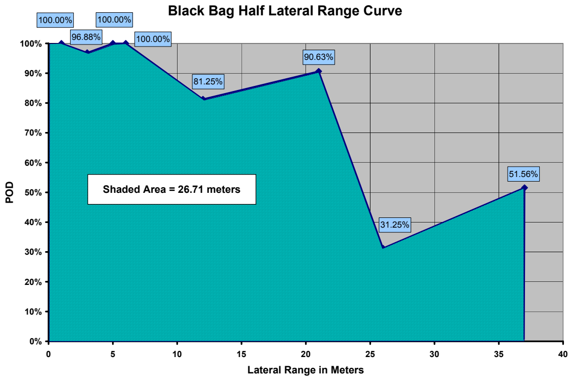
Figure 21. Black Garbage Bag Half Lateral Range Curve— W = 53 meters. (Area under this portion equals one-half effective sweep width value.)
