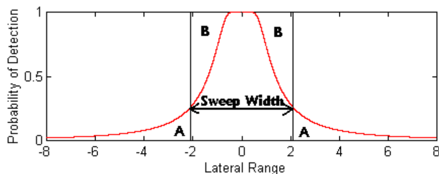
Figure 2. A Lateral Range Curve. The number of missed detections (B) inside the effective sweep width equals the number of detections (A) that occur outside the sweep width.
