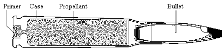
Figure 5. Cartridge Components
