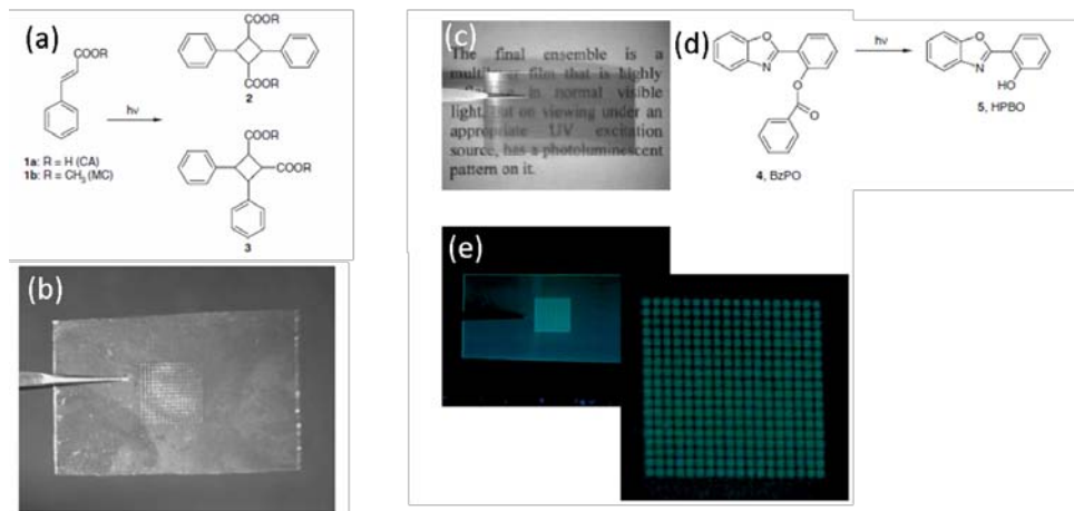
Figure 13. Depiction of photopatterned films using a refractive index changing additive and a fluorescent dye. (a) Photodimerization of CA into (2) truxinic acid and (3) truxillic acid. (b) Picture of a photopatterned coextruded film containing PMMA layered against PMMA with 12 wt% CA. (c) Photograph of a 1024 layered PMMA/BzPO-PC film containing 0.5 wt% BzPO exposed to 254 nm UV light through a checkerboard mask for 15 min. (d) Photochemically induced cleavage of 2-(2'-benzoylphenyl)benzoxazole (BzPO) under formation of 2-(2'-hydroxyphenyl)benzoxazole (HPBO). (e) 1024 layered PMMA/BzPO-PC film shown under 365 nm UV light. The inset shows higher magnification.
