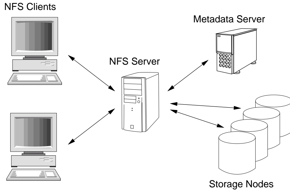
Figure 4.1: NFS server as storage system client
