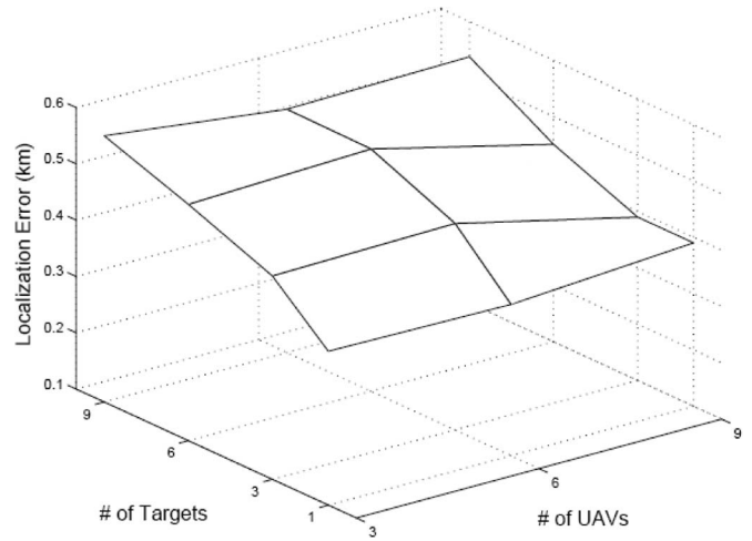
Fig. 12. Plot of the average localization error in kilometers when the number of UAVs changes from three to nine and the number of targets changes from one to nine using a 7^\circ accurate sensor.
