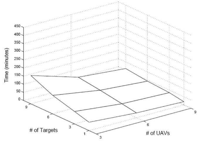
Fig. 13. Plot of the average total search/localization time in minutes when searching a 50 \times 75 km area as the number of UAVs changes from three to nine, and the number of targets changes from one to nine.
