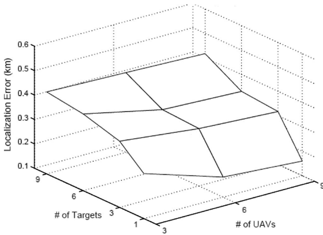
Fig. 11. Plot of the average localization error in kilometers when the number of UAVs changes from three to nine and the number of targets change from one to nine using a 1^\circ accurate sensor.
