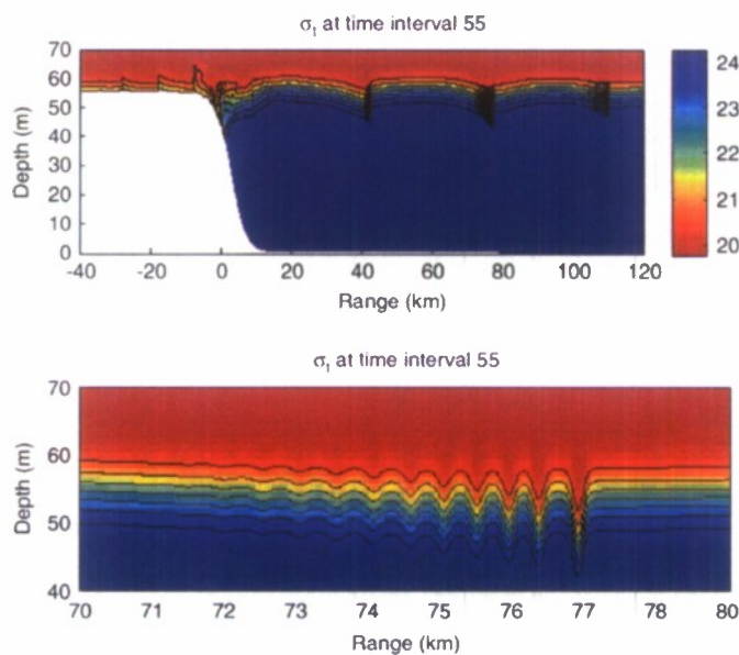
Fig. 9. Case 6 in Table 2. This case has a lower barotropic tidal forcing velocity, U_0 = .3 m/s, relative to case 1. Predicted density field at 55 h. Upper panel shows predicted density structure. Lower panel shows an expanded view of second solitary wave train. Note a decrease in number of solitary waves in train and their amplitudes relative to case 1.
