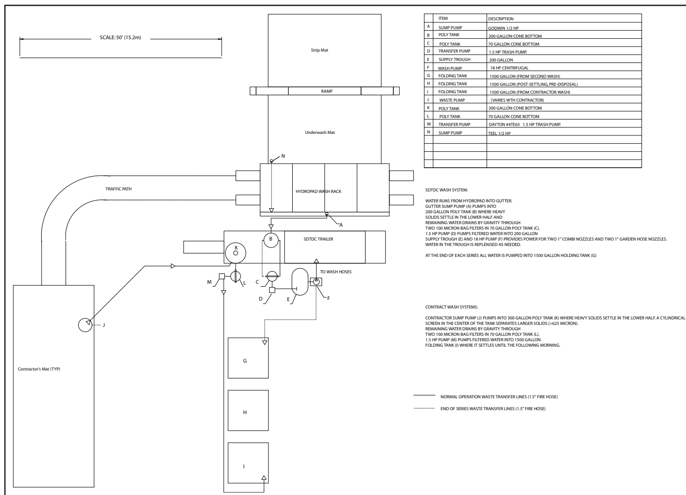
Figure 8—Waste recovery drawing.
