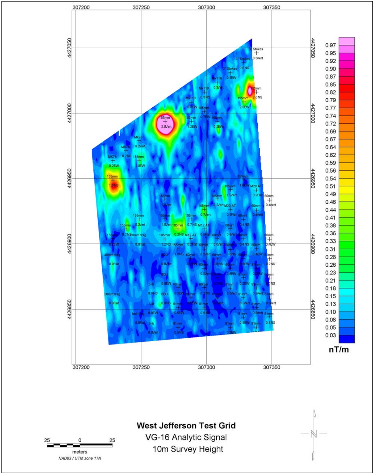
Figure 4-4b. VG-16 airborne analytic signal results for 10m altitude from the West Jefferson Test Site.
