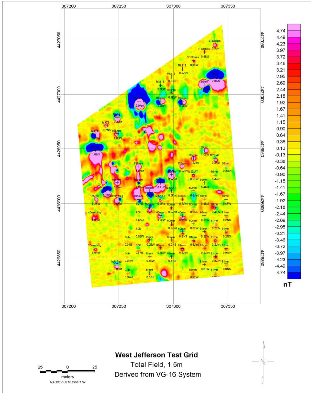
Figure 4-1a. VG-16 airborne vertical magnetic gradient results for 1.5m altitude from the West Jefferson Test Site.
