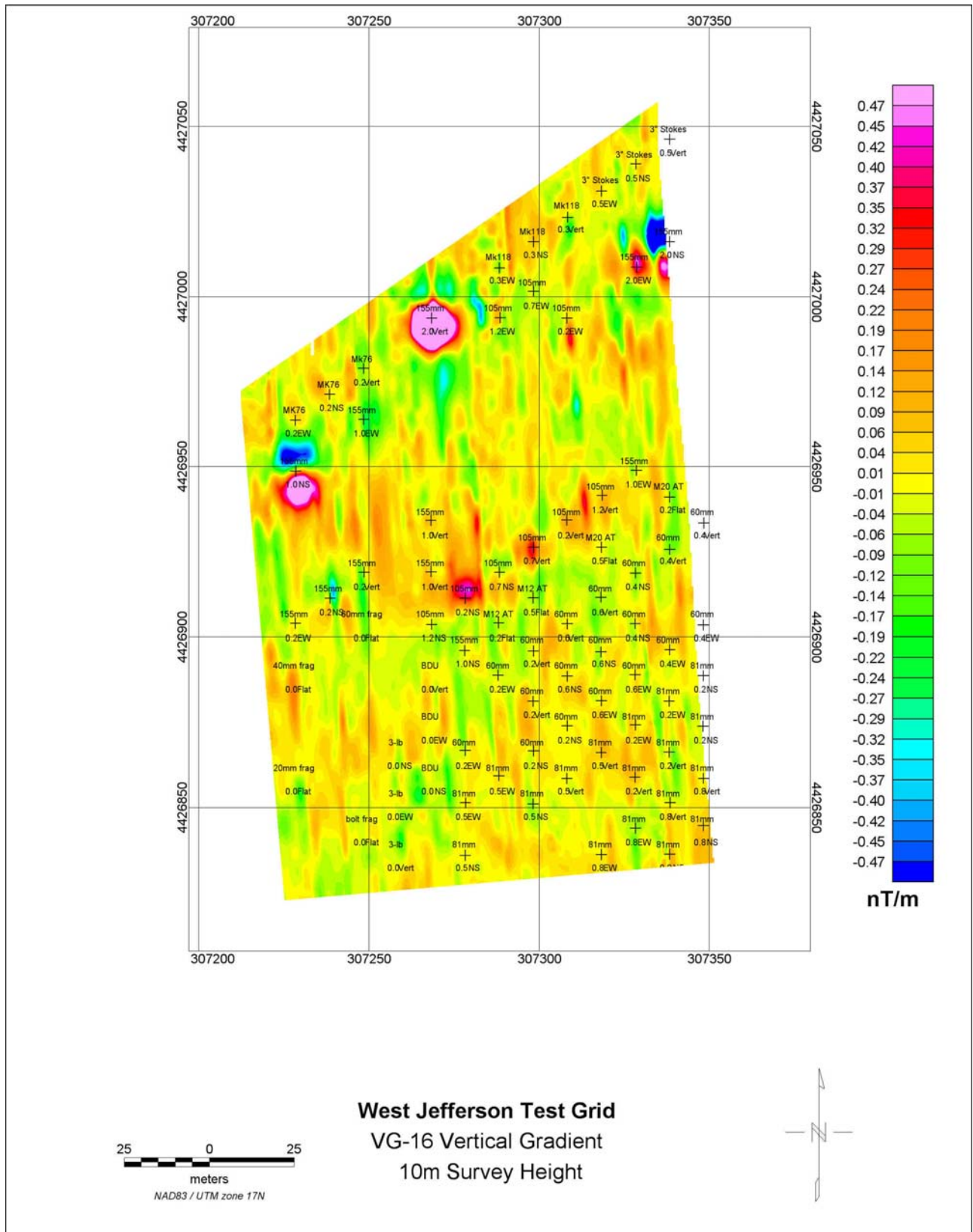
Figure 4-4a. VG-16 airborne vertical magnetic gradient results for 10m altitude from the West Jefferson Test Site.
