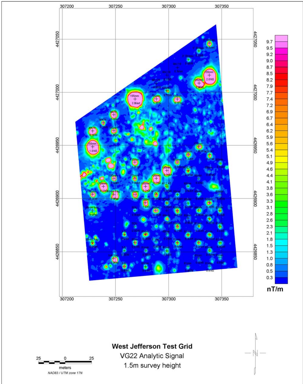
Figure 4-5b. VG-22 airborne analytic signal results for 1.5m altitude from the West Jefferson Test Site. The color bar used here is the same as in Figure 4.1b, as both data sets were acquired at similar altitude.
