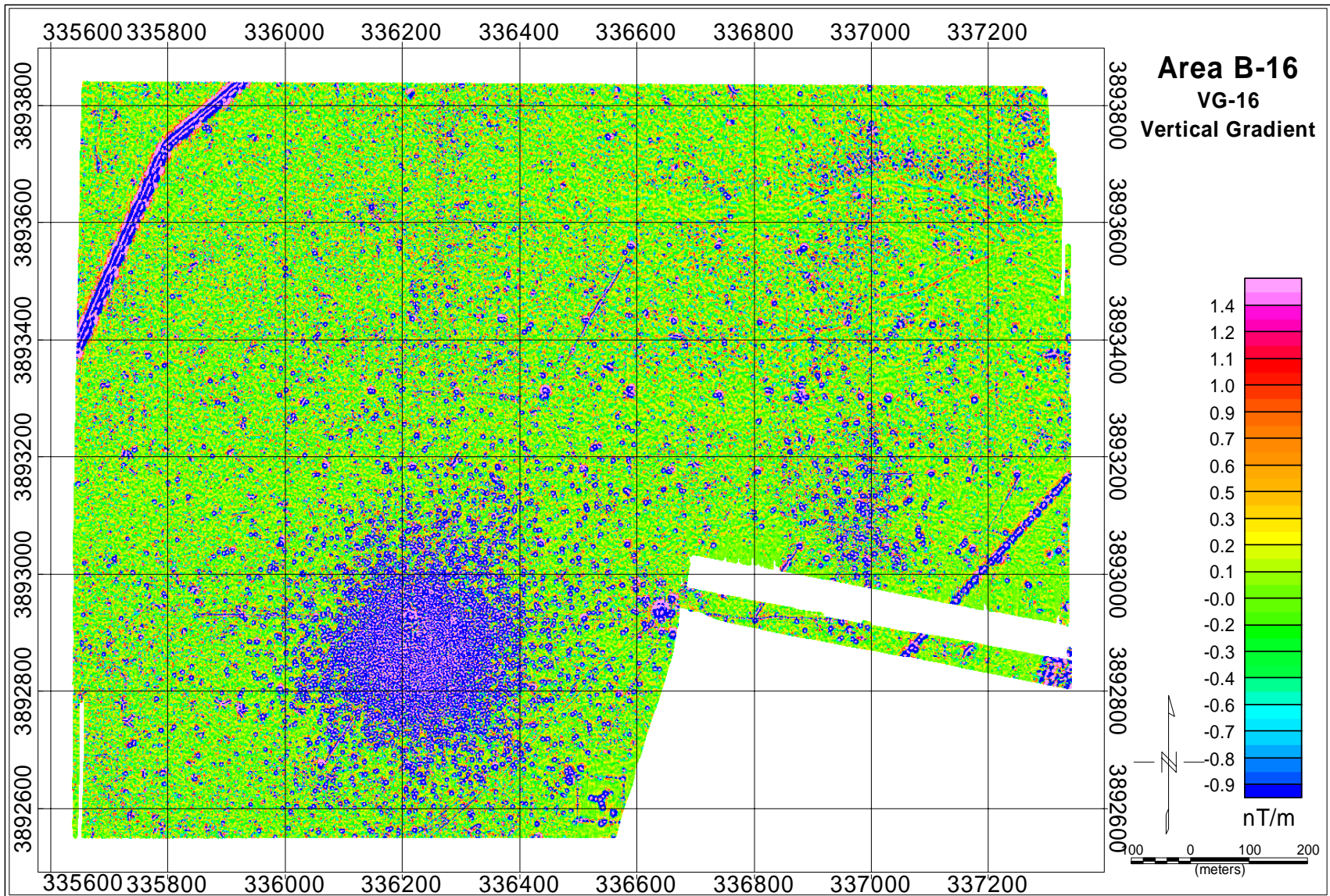
Figure 4-28. VG-16 vertical magnetic gradient map of North Area B at FKPB.
