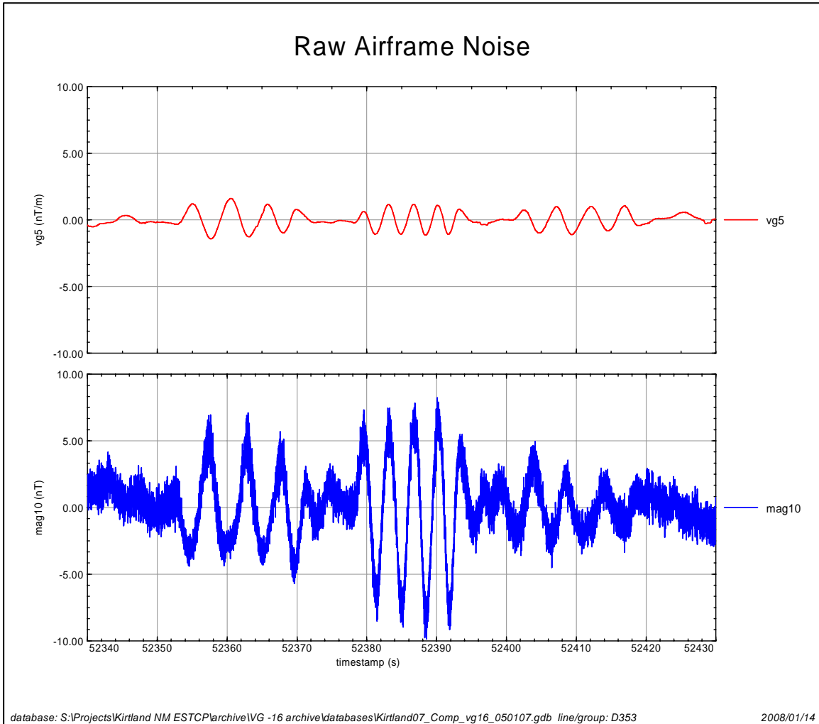
Figure 4-16. Raw airframe noise prior to compensation over a 90sec data sample. The vertical gradient demonstrates a 6.6x reduction in noise. The high frequency noise observable in the total field profile is rotor noise.
