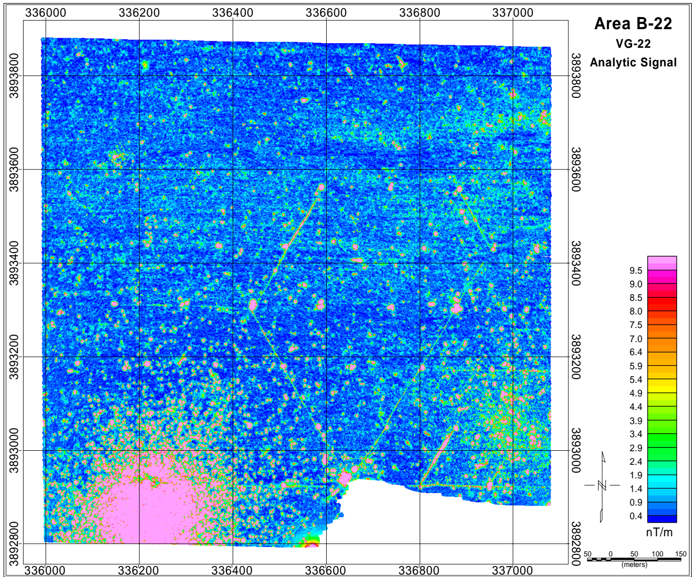
Figure 4-31. VG-22 analytic signal map of North Area B at FKPBR.
