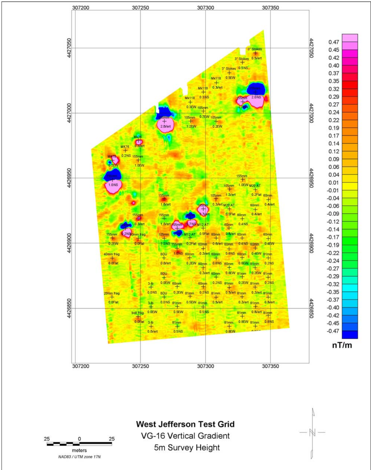
Figure 4-3a. VG-16 airborne vertical magnetic gradient results for 5m altitude from the West Jefferson Test Site. Note that the color bar is different from Figures 4.1a, because of the weaker signal at increased altitude.
