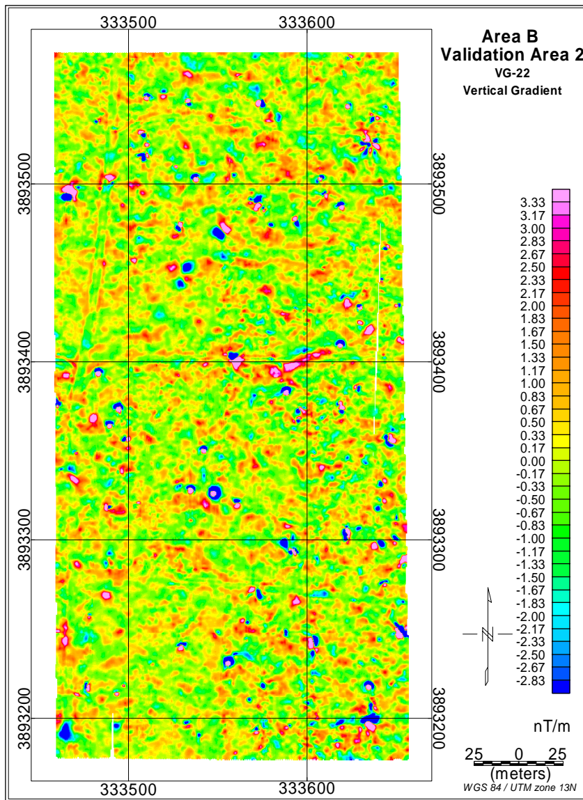
Figure 4-35. VG-22 maps for Validation Area 2, Area B, at FKPBR: a) vertical magnetic gradient map; and b) analytic signal.
