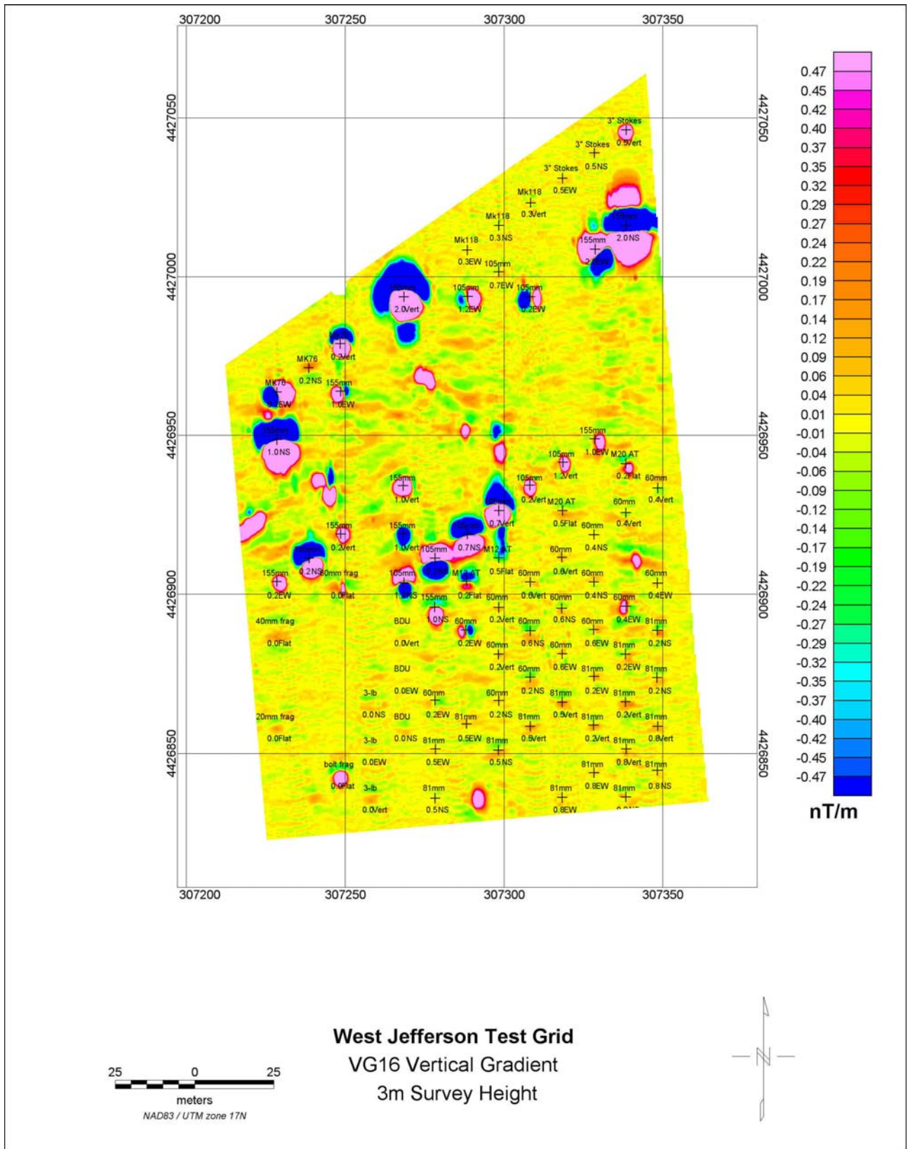
Figure 4-2a. VG-16 airborne vertical magnetic gradient results for 3m altitude from the West Jefferson Test Site. Note that the color bar is different from Figure 4.1a because of the weaker signal at increased altitude.
