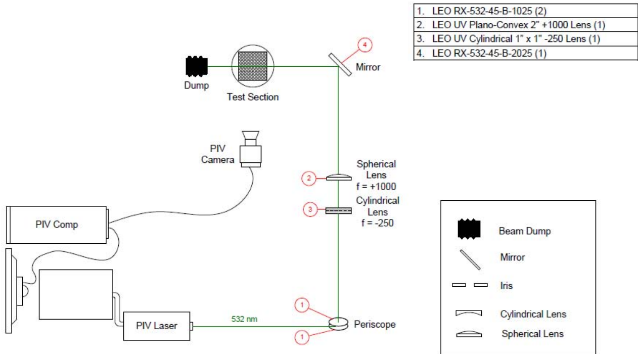
Figure 23. PIV setup
