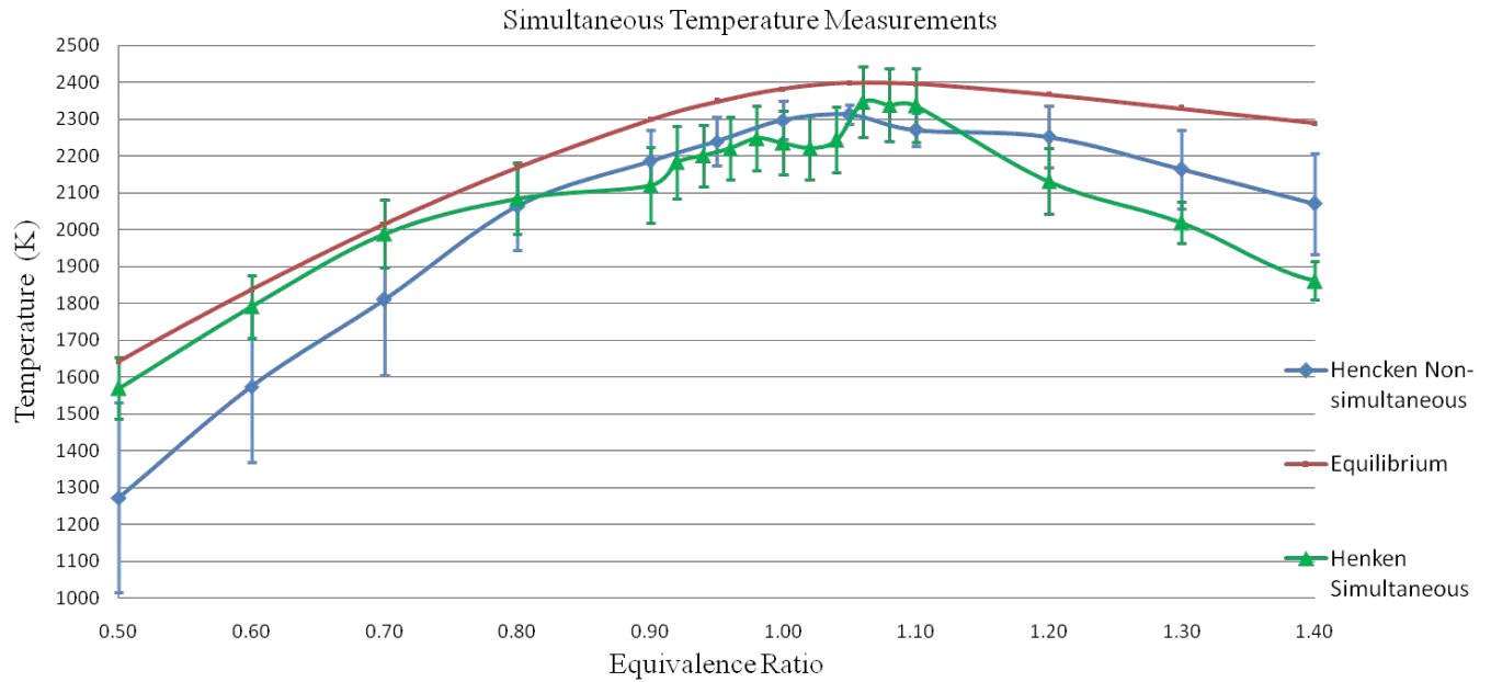
Figure 52. Simultaneous temperature measurements of Hencken flame
