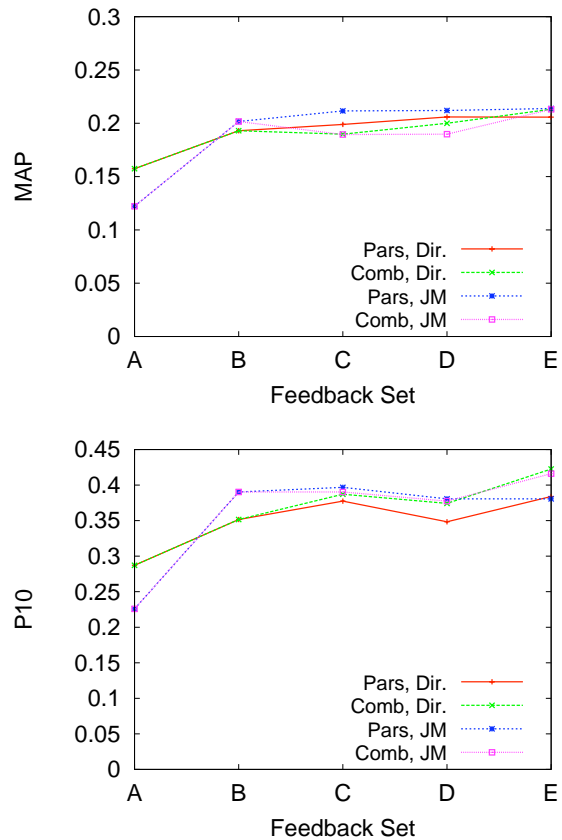
Figure 2: Official results: MAP and P10
