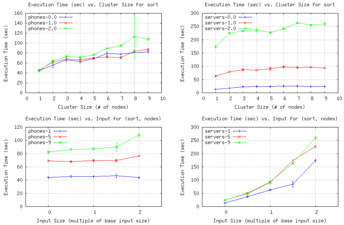
Figure 6.8: Execution time vs. number of nodes (top) and input size (bottom) for phones (left) and servers (right), Sort benchmark
