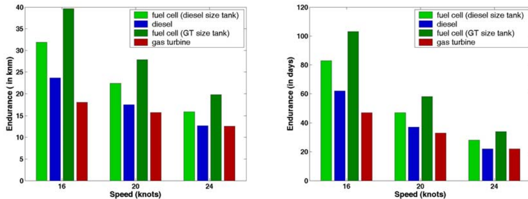
Figure 13: Comparison of endurance for the fuel cell powered LMSR with the diesel and gas turbine powered LMSRs in terms of distance and days traveled by the vessel with full tank of fuel.
