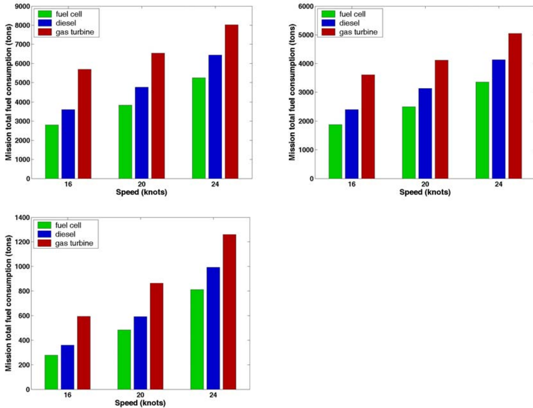
Figure 12: Fuel consumptions for three different mission scenarios and three power plants.
