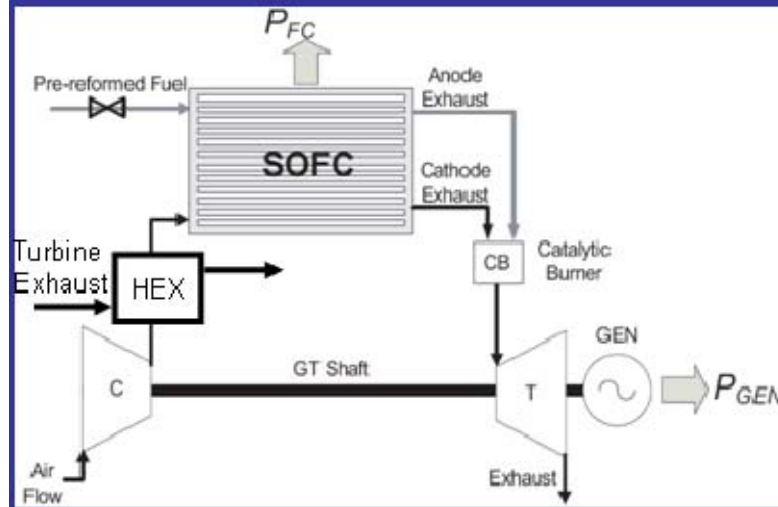
Figure 5: Schematic of the hybrid SOFC-GT system.
