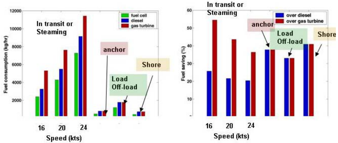
Figure 10: Fuel consumption for different operating modes.
