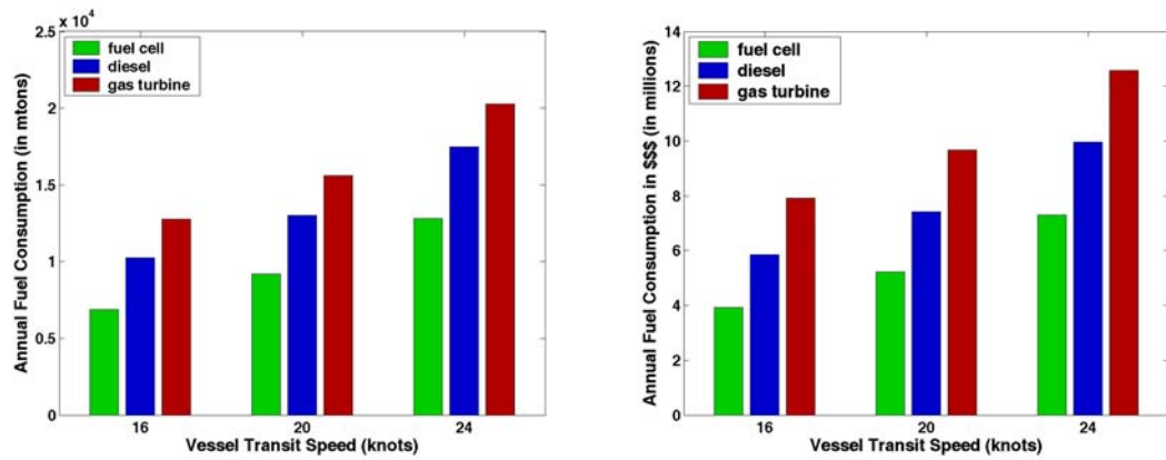
Figure 11: Annual fuel consumptions for three different power plants.
