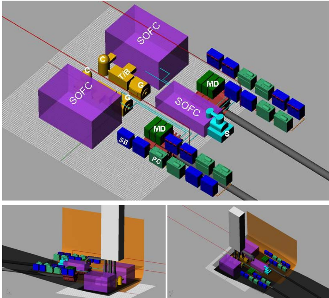
Figure 14: Machinery arrangement of configuration A.
