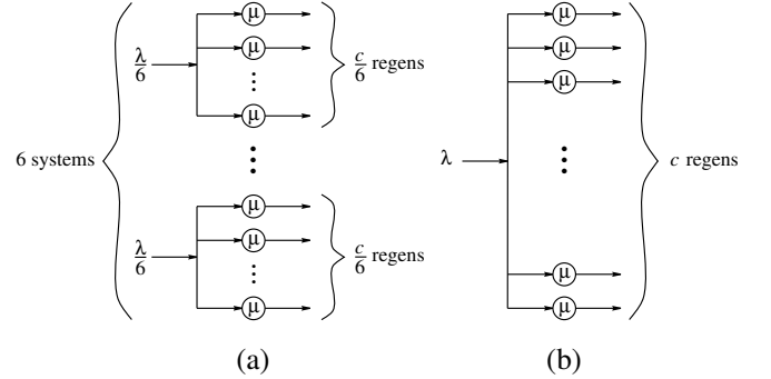
Fig. 4. (a): Queuing model for the SART switch using 6 sets of c' regenerators, where the probability that an arrival will be directed to a given set of servers is uniform. (b): Queuing model for the DART switch using c regenerators with single arrival source.
