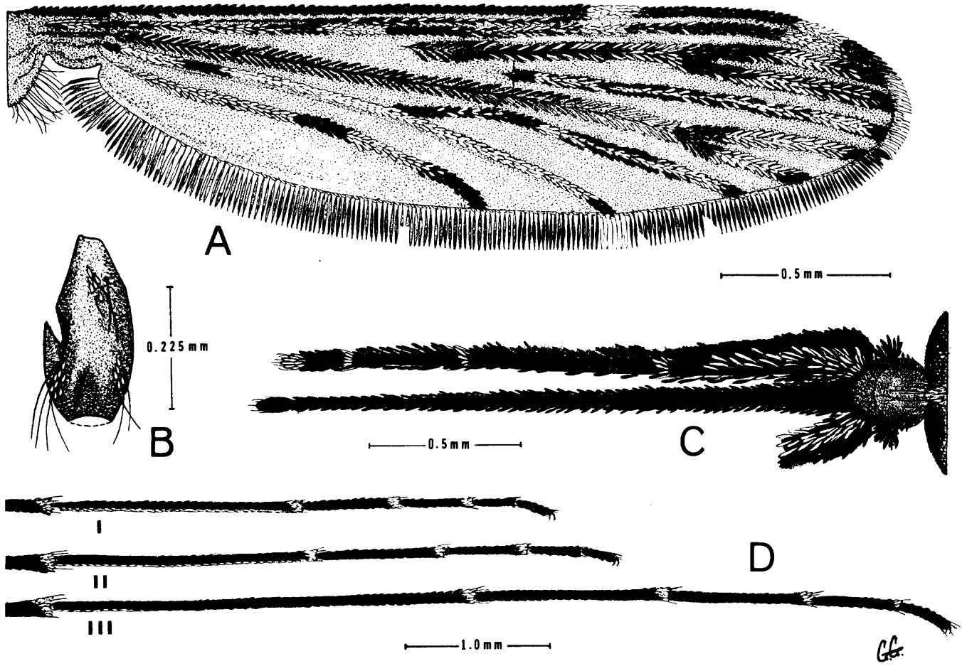
Fig. 1 Anopheles (Anopheles) sinensis Wiedemann. Lectotype female. A. dorsum of right wing; B. lateral view of right mid coxa; C. dorsum of proboscis, right palpus and clypeus; D. lateral view of fore, mid and hind tarsomeres.
