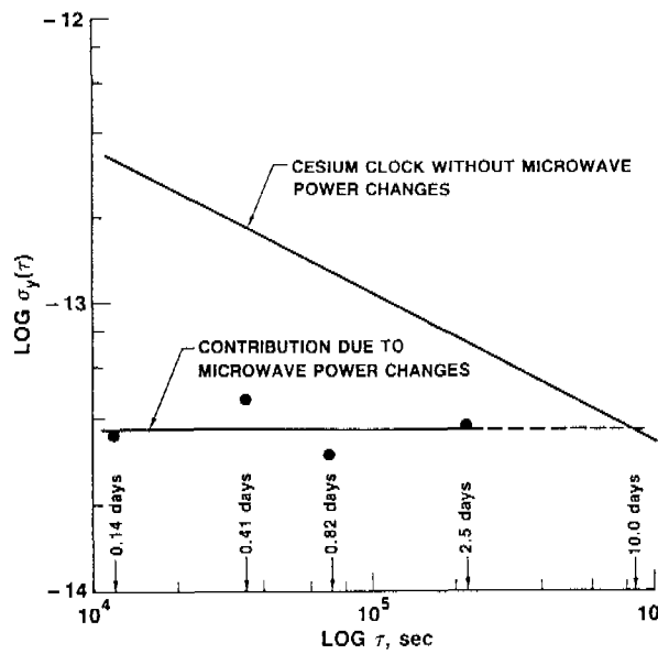
Fig. 14. A Plot of the Calculated Contribution of Microwave Power Changes to the Allan Standard Deviation for Cesium Clock No. 1.
