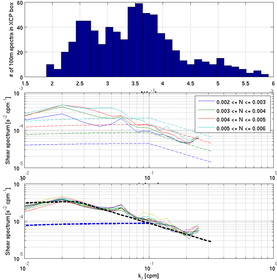
Figure 4: (upper panel) Histogram of buoyancy frequency ( N ) values corresponding to each 100m segment of XCP shear profiles. Most of the values lie between 0.002 and 0.004 s^{-1} , with a scattering of higher values. (Middle panel) Solid lines show 100m shear spectra bin-averaged by N . Dashed lines show corresponding Garrett-Munk spectra (Gregg and Kunze, 1991). Measured spectra do not scale with N as expected, implying relatively higher energy in the lower (less-stratified) part of the water column. (Bottom panel) Solid lines show 100m shear spectra averaged over each XCP station in the 3x3 survey. The shapes are very similar from one station to another and agree well with a modified GM spectrum (black dashed line) adjusted to an energy level 4 times higher than the open ocean value (blue dashed line), along with a saturation-range roll-off at a correspondingly lower wavenumber. The peak at 0.06 cpm is believed to be an instrument artifact. GM spectra were plotted with the help of Jody Klymak's Matlab toolbox ( http://hornby.seos.uvic.ca/~jklymak/GarrettMunkMatlab/ ).
