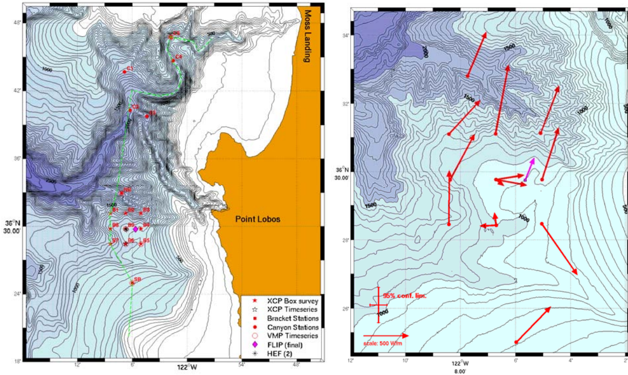
Figure 1: (left panel) Chart showing the locations of timeseries stations occupied over the slope west of Point Lobos and northward into Monterey Canyon during the 2006 profiling survey on the R/V Point Sur . Bathymetric contours from a 250m (horizontal) resolution database are shown at a vertical interval of 50m. The green line connecting a south-to-north subset of the stations is used to generate the section shown in Fig.3. (Right panel) Enlarged view of the high-resolution survey site near FLIP. Bathymetric contours are now from a 40m database. Semidiurnal energy flux vectors from the XCP survey (red arrows) show a generally northward flux of around 500 W/m except at the central, south, and southeastern stations, which show weak or southward flux. The maximum semidiurnal flux from FLIP (most comparable to the XCP survey at spring tide) is only about 200 W/m (magenta arrow), but is consistent with an average of the two adjacent stations. 95% confidence limits on the XCP flux estimates (scale bar in lower left corner) are approximately \pm 200 W/m in the north–south direction, and much less for the FLIP estimate.
