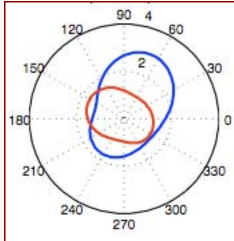
Figure 6: Mode-1 M_2 plane wave fit results for HF Radar velocities over the entire Fig.5 domain, following the altimeter techniques of Zhao and Alford (2009). The blue line shows the north-south velocity amplitude as a function of wave direction, and the red line shows the east-west velocity amplitude. Even when applied over the entire region, a north-northeast propagating wave is evident.
