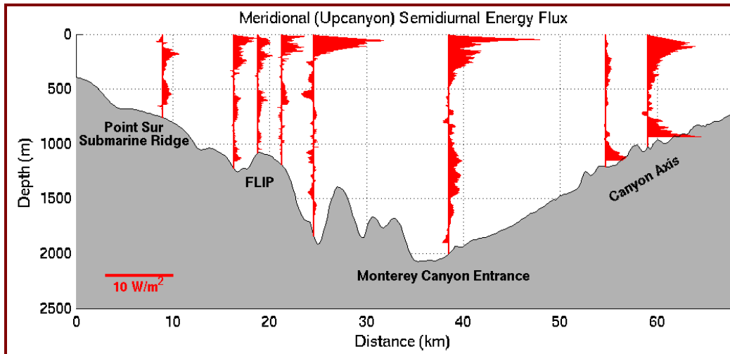
Figure 3: A section along the green line in Fig. 1, showing the bathymetry and along-section energy flux profiles from the ridge west of Point Sur (left side), through the survey box around FLIP, and up the axis of Monterey Canyon (right side). Energy flux is enhanced in the upper and lower water column due to the overall low-mode internal tide. The more complicated picture in the lower water column near the FLIP site is symptomatic of additional local generation.
