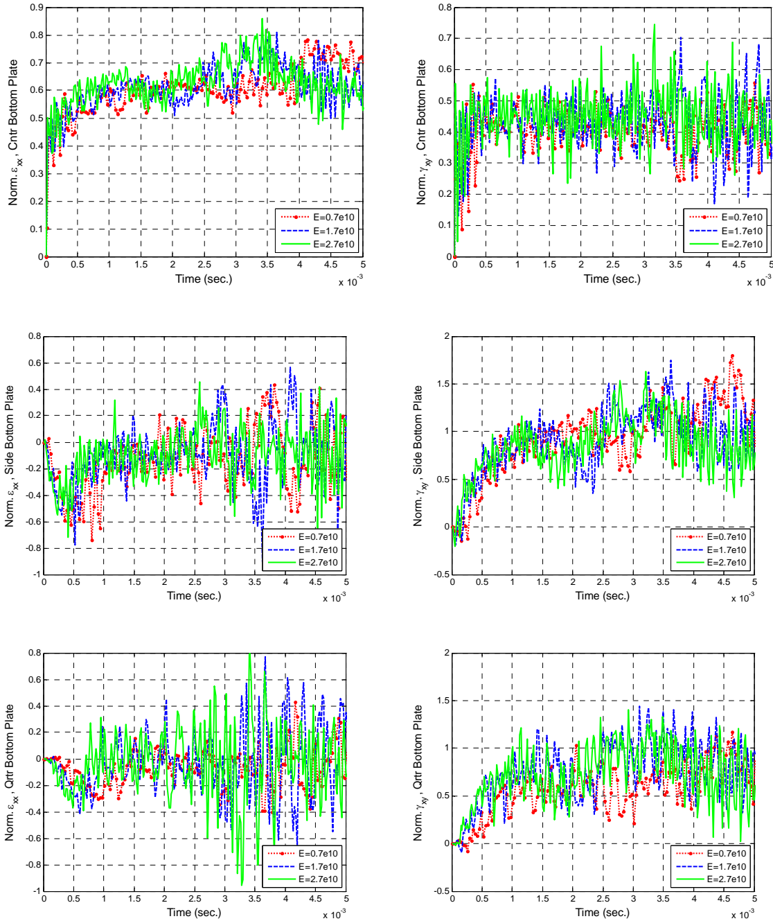
Figure 36. Normal and Shear Strains for Comparison of Different Elastic Modulus for Two-sided Wet Structure with Concentrated Force and Clamped Boundary (Alternate Normalization)
