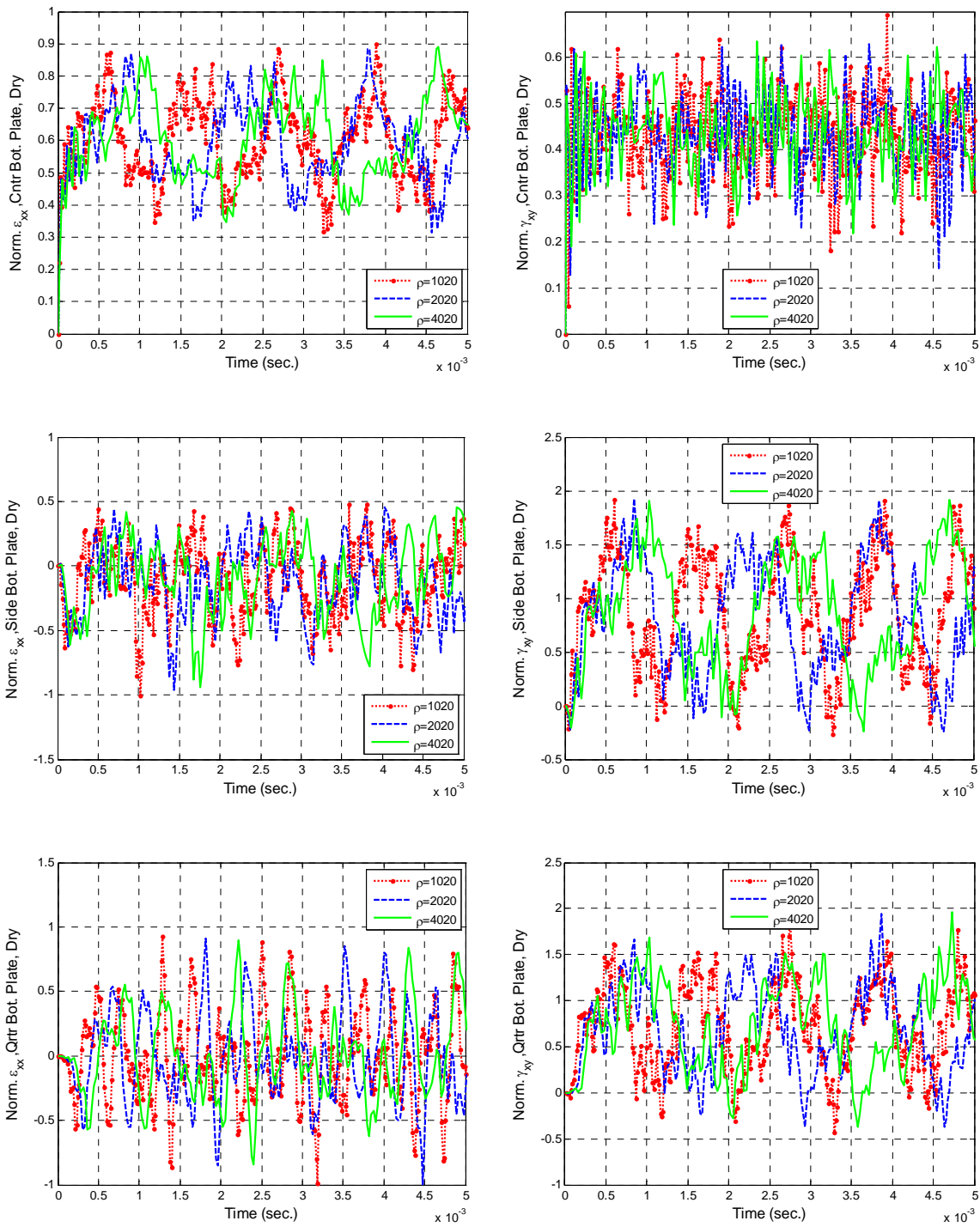
Figure 75. Normal and Shear Strains for Comparison of Different Density for Dry Structure with Concentrated Force and Clamped Boundary
