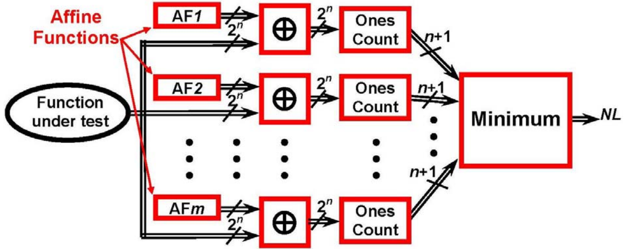
Figure 1. Process for Computing Nonlinearity of a Function (From [17])
