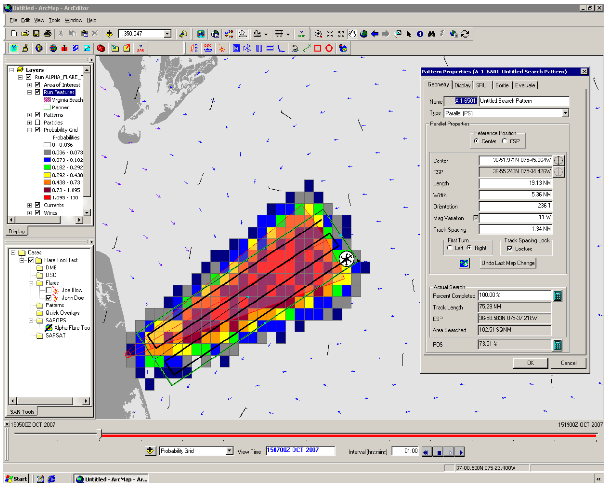
Figure I-21: SAROPS Search Plan (CST Two Hours After Flare Sighting)
