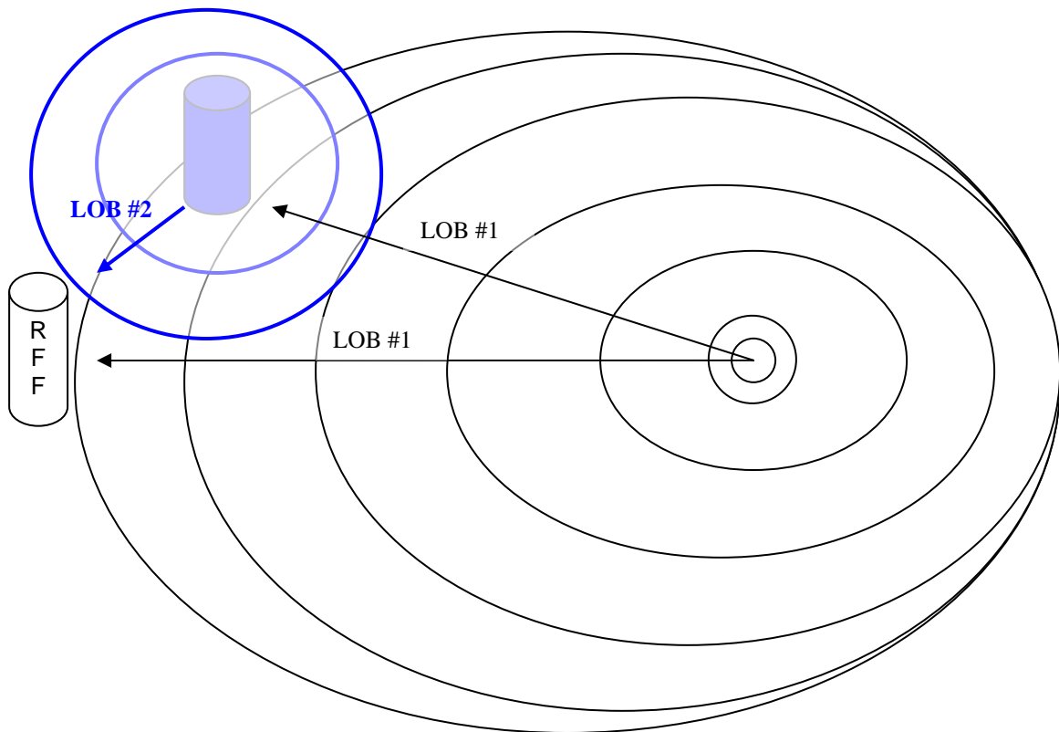
Figure 2-5 Transmission Bounce
