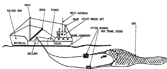
Side Trawler
