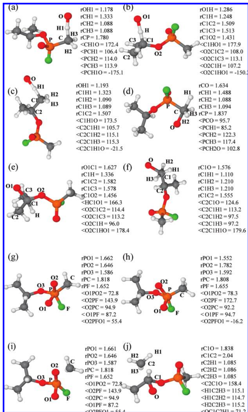
Figure 4. Structures for O( 3 P) + sarin: (a) hydrogen abstraction reaction (7) transition state, (b) hydrogen abstraction reaction (8) transition state, (c) hydrogen abstraction reaction (9) transition state, (d) hydrogen elimination reaction (10) transition state, (e) hydrogen elimination reaction (11) transition state, (f) hydrogen elimination reaction (12) transition state, (g) methyl elimination reaction (13) first transition state, (h) methyl elimination reaction (13) stable intermediate, (i) methyl elimination reaction (13) second transition state, and (j) methyl elimination reaction (14) transition state. All bond angles (in degrees) and lengths (in angstroms) are from the CBS-QB3 calculations. Complete geometric information for these transition states is given in the Supporting Information.
