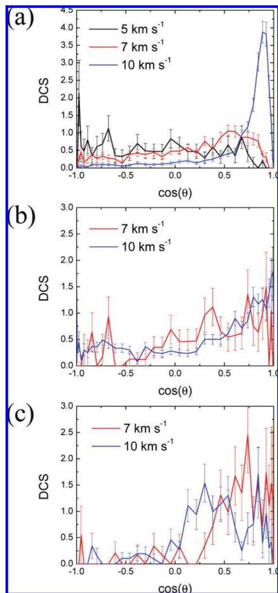
Figure 7. The angular distributions of the scattering products of the O( 3 P) + sarin reaction plotted as normalized differential cross sections, ( DCS = 1/\sigma d\sigma/(\sin \theta d\theta) , d\theta = 5^\circ ), at 5, 7, and 10 km s -1 : (a) hydrogen abstraction, (b) hydrogen elimination, and (c) methyl elimination. The scattering angle \theta is defined as the angle between the incident O atom and the OH, H, or CH 3 product, respectively, in the center-of-mass frame.
