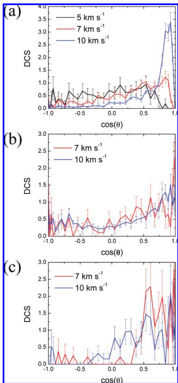
Figure 6. The angular distributions of the scattering products of the O( 3 P) + DMMP reaction plotted as normalized differential cross sections, ( DCS = 1/\sigma d\sigma/(\sin \theta d\theta) , d\theta = 5^\circ ), at 5, 7, and 10 km s -1 : (a) hydrogen abstraction, (b) hydrogen elimination, and (c) methyl elimination. The scattering angle \theta is defined as the angle between the incident O atom and the OH, H, or CH 3 product, respectively, in the center-of-mass frame.
