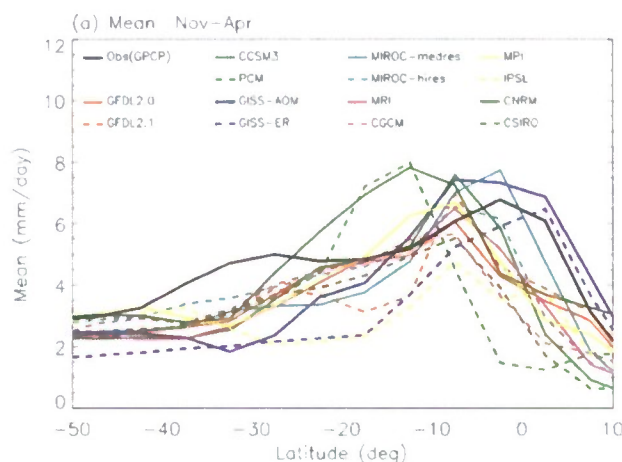
FIG. 2. Meridional profile of southern summer (November–April) seasonal mean precipitation averaged between 30° and 60°W for the observations and the 14 models.
