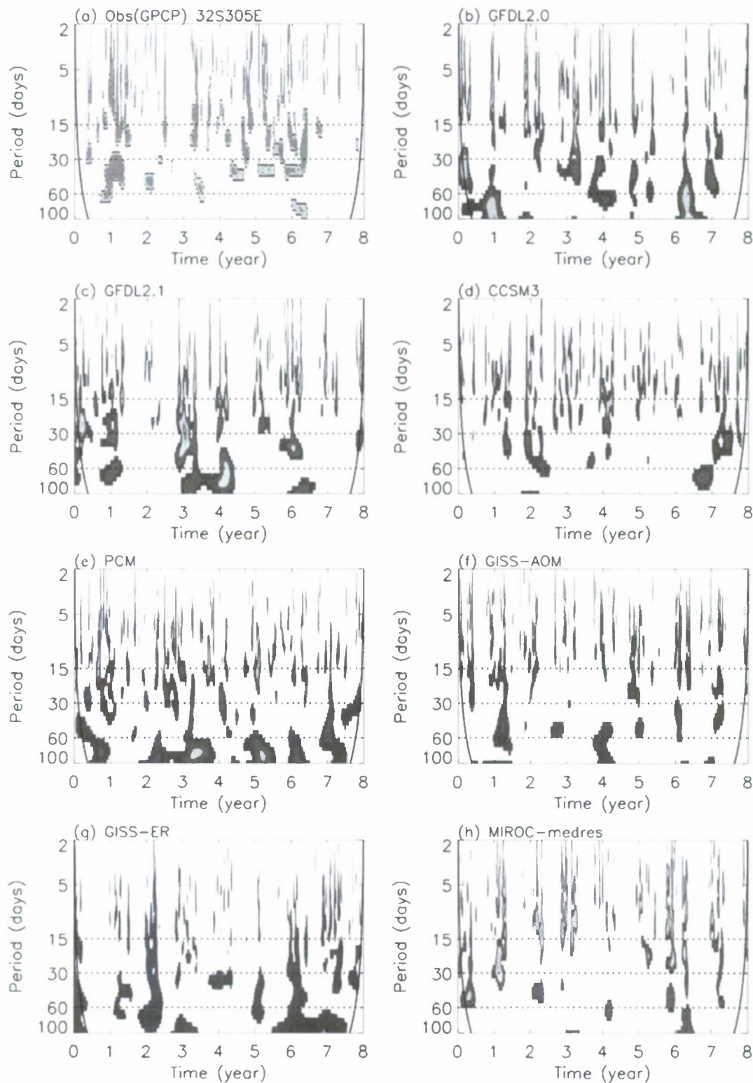
FIG. 5. Wavelet spectrum of precipitation averaged between 30°–35°S, 50°–60°W. Only spectral peaks above the 95% confidence level are plotted.
