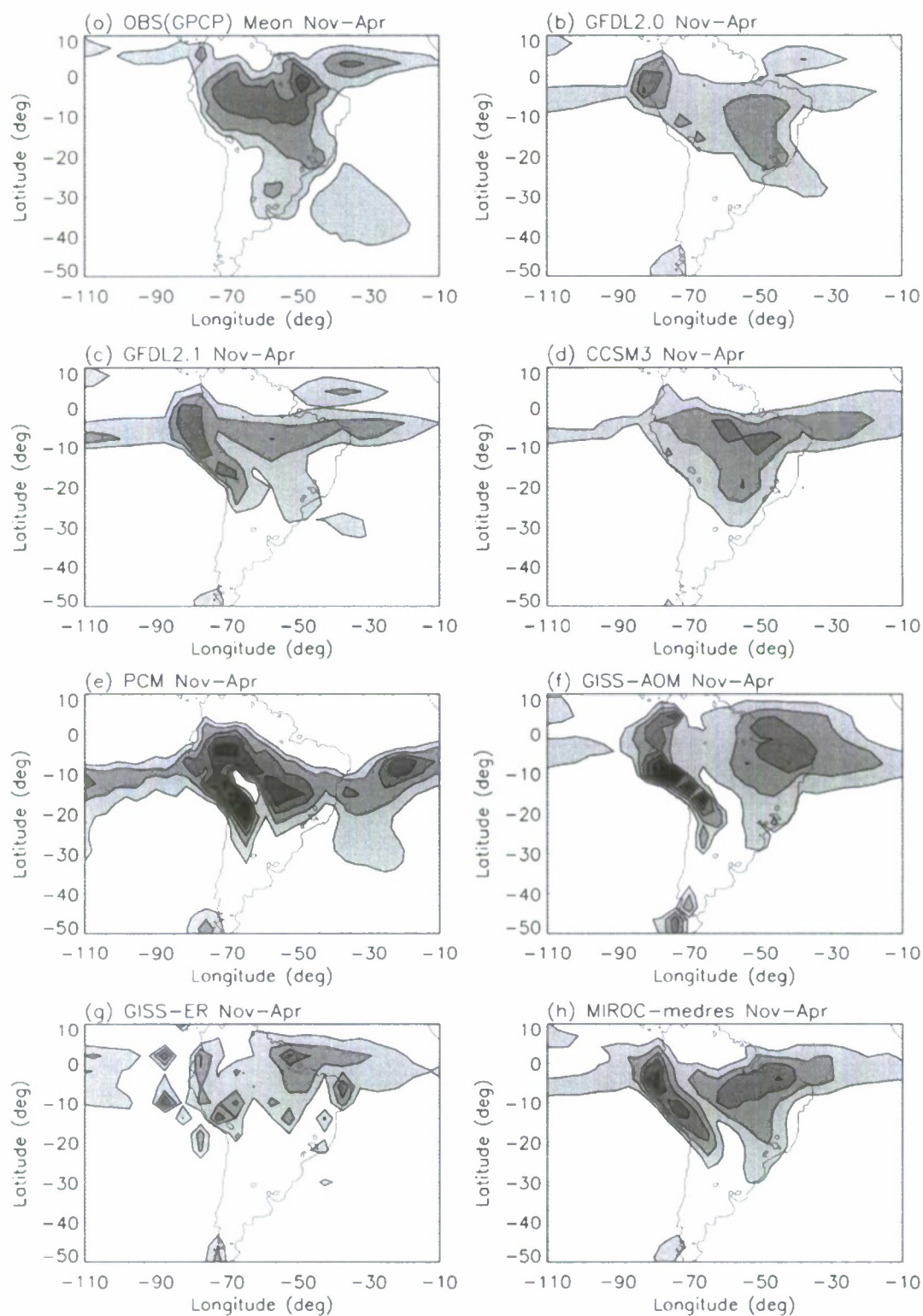
FIG. 1. Southern summer (November–April) seasonal mean precipitation for observation and 14 IPCC AR4 models. The first contour is 4 \text{ mm day}^{-1} and the contour interval is 2 \text{ mm day}^{-1} .
