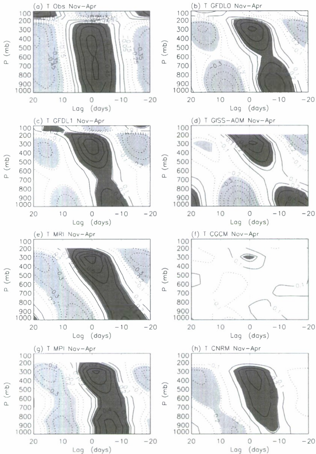
FIG. 8. Lag correlation of temperature averaged between 20^{\circ} – 30^{\circ} S and 50^{\circ} – 60^{\circ} W vs the 40-day band precipitation anomaly at the same location for observation (NCEP–NCAR reanalysis) and the seven models. Shading denotes the area where correlation is above the 95% confidence level, with dark (light) shading for positive (negative) correlation.
