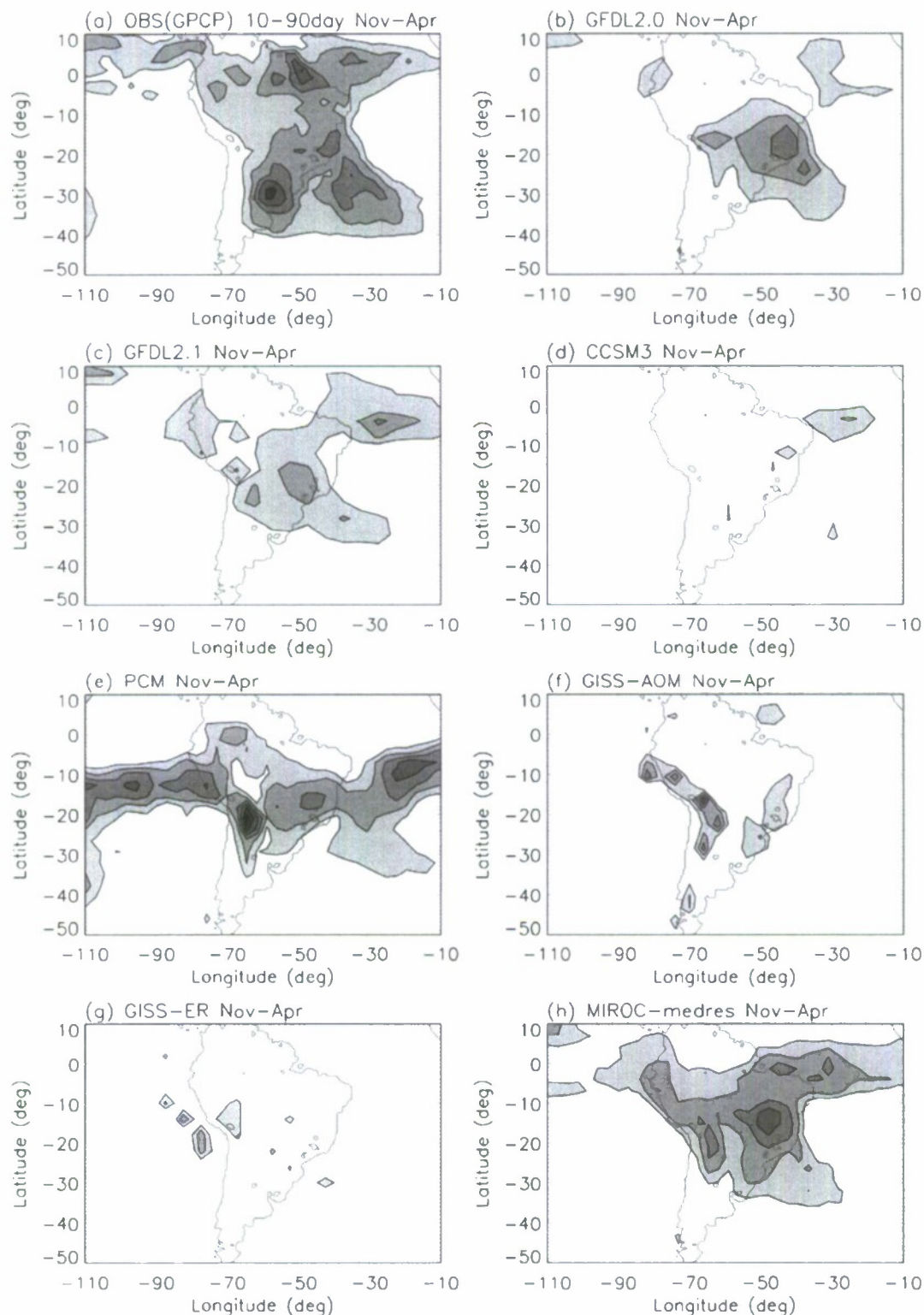
FIG. 3. Horizontal distribution of the standard deviation of total intraseasonal (10–90 day) precipitation anomaly during northern summer (November–April). The first contour is 3 \text{ mm day}^{-1} and the contour interval is 1 \text{ mm day}^{-1} .
