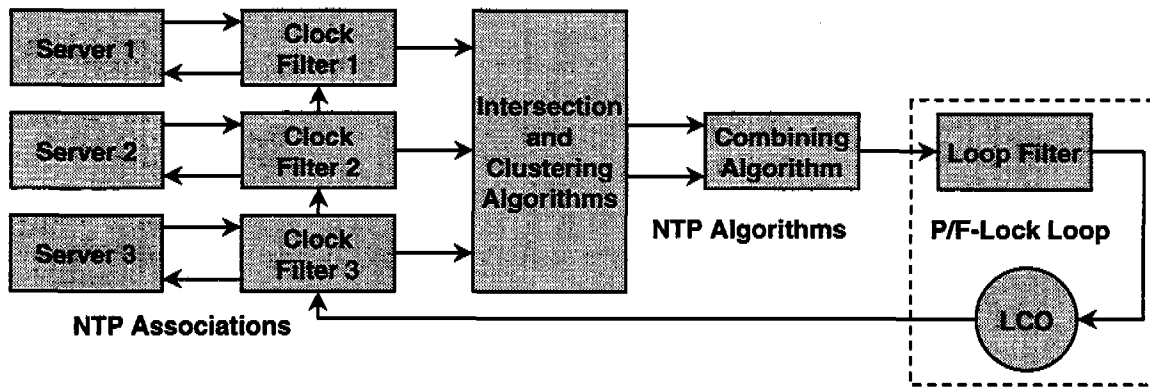
Figure 1. NTP Server Functional Organization
