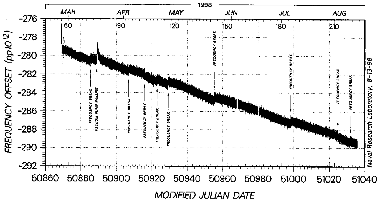
Fig. 8. RAFS No. 28 Frequency Offset Weeks 48 - 70
