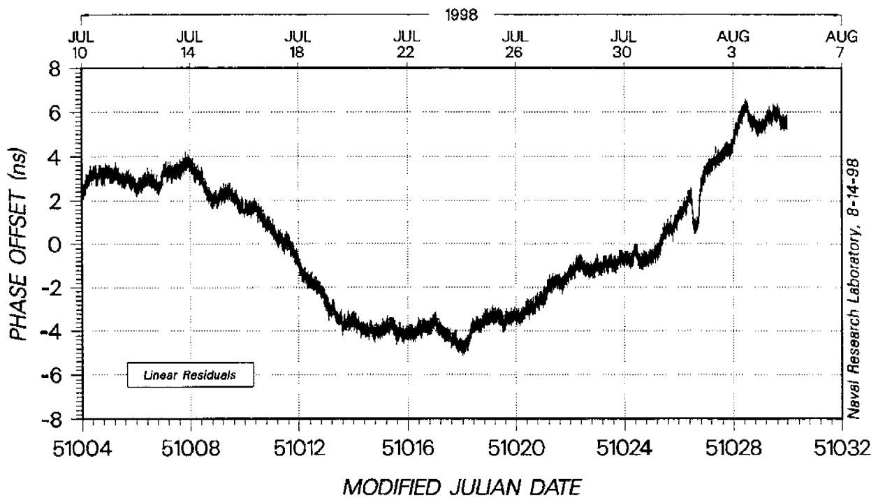
Fig. 15. RAFS No. 30 TKSS Phase Offset
