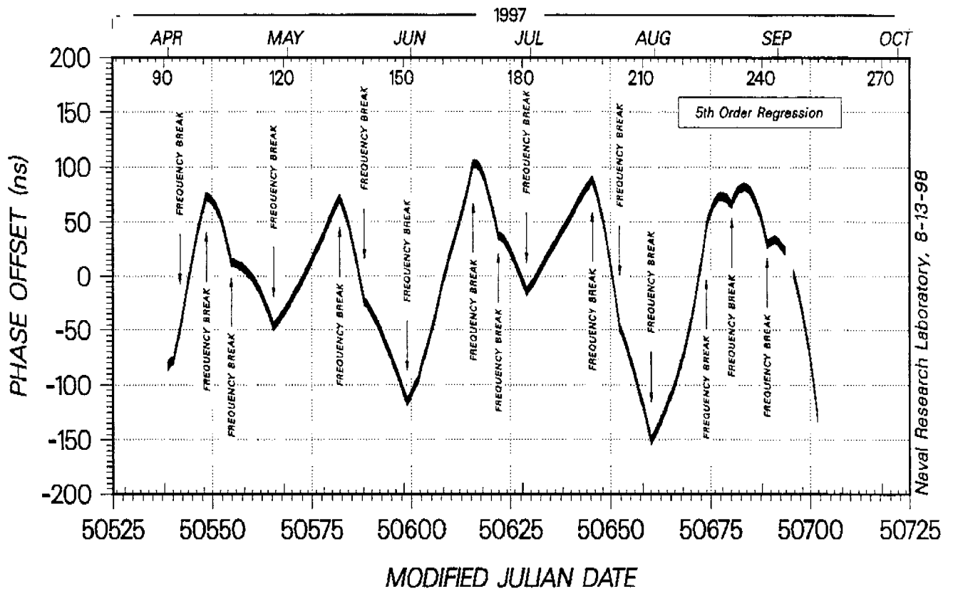
Fig. 3. RAFS No. 28 Phase Offset Residuals Weeks 1 - 24
