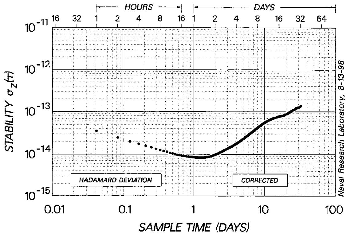
Fig. 7. RAFS No. 28 Stability Weeks 1 - 47
