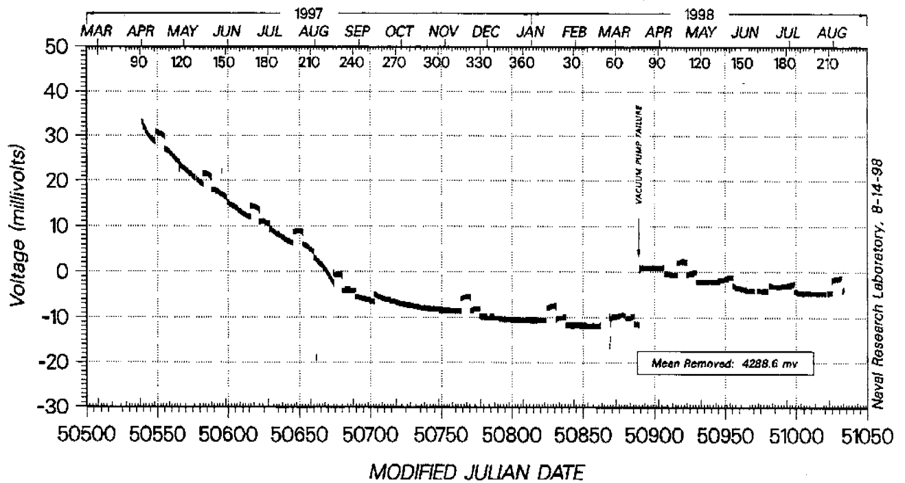
Fig. 4. RAFS No. 28 Lamp Output Voltage
