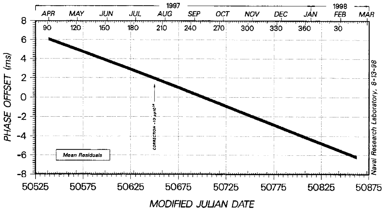
Fig. 11. RAFS No. 30 Corrected Phase Weeks 1 - 47
