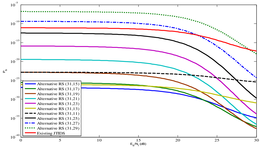
Figure 14. Performance of 32-ary CCSK using concatenated coding in both AWGN and PNI for \rho=0.01 , coherent demodulation, hard decision decoding and E_b / N_0 = 10 dB.
