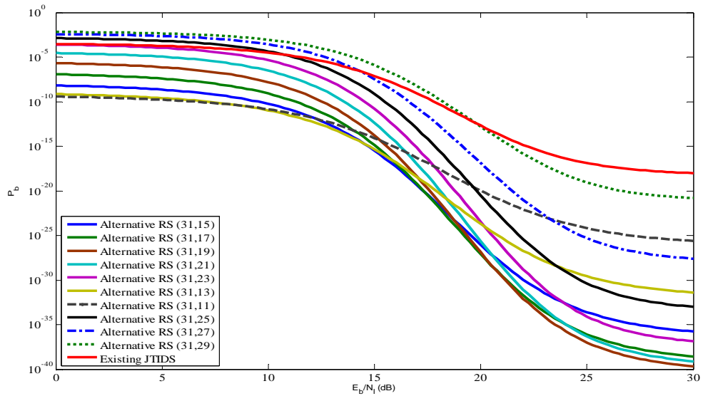
Figure 12. Performance of 32-ary CCSK using concatenated coding in both AWGN and PNI for \rho=0.1 , coherent demodulation, hard decision decoding and E_b / N_0 = 10 dB.
