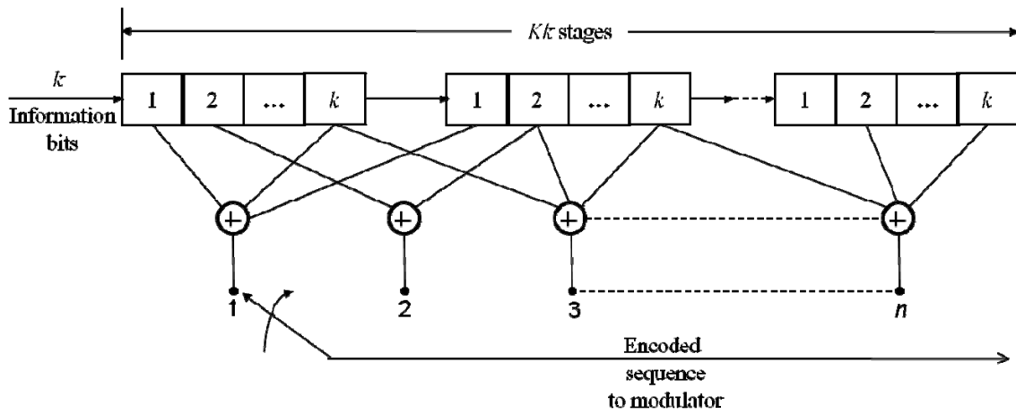
Figure 3. Convolutional encoder [From 7]
